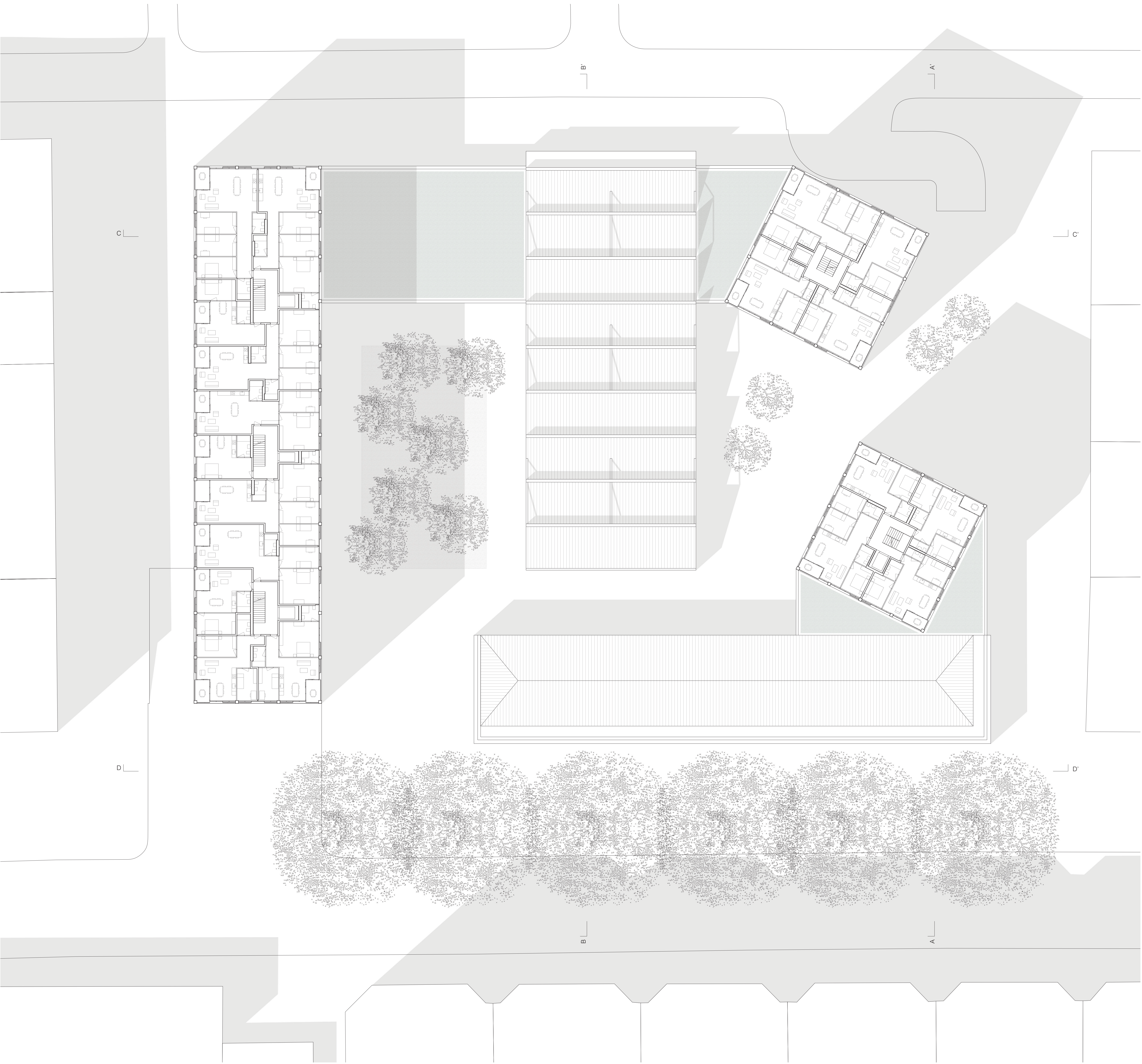
Plan type: logements 1:200
