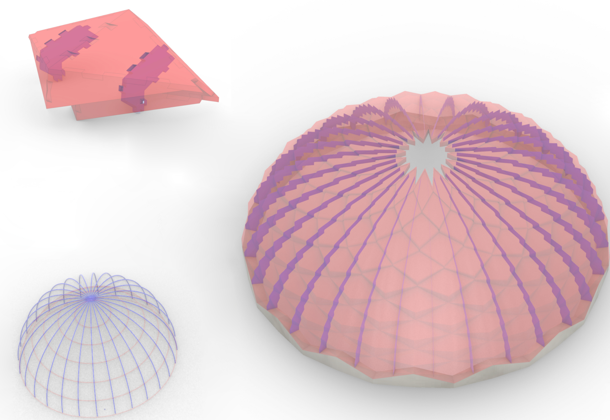
Structural Scheme
