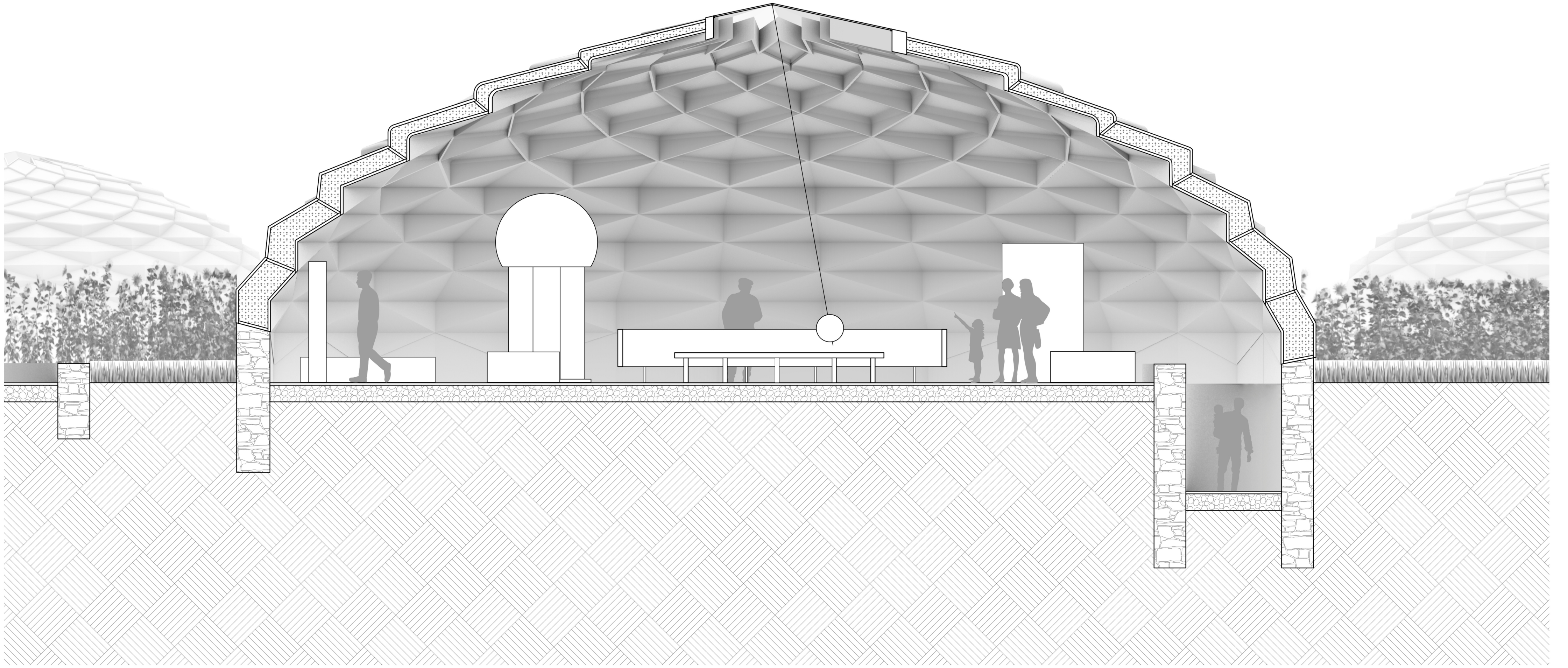
Section 1:50
