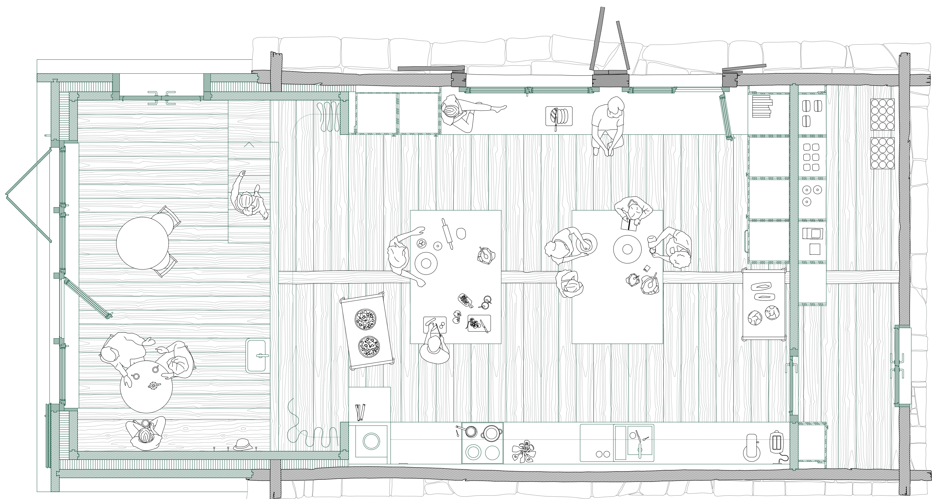
Floor plan common kitchen 1:33
