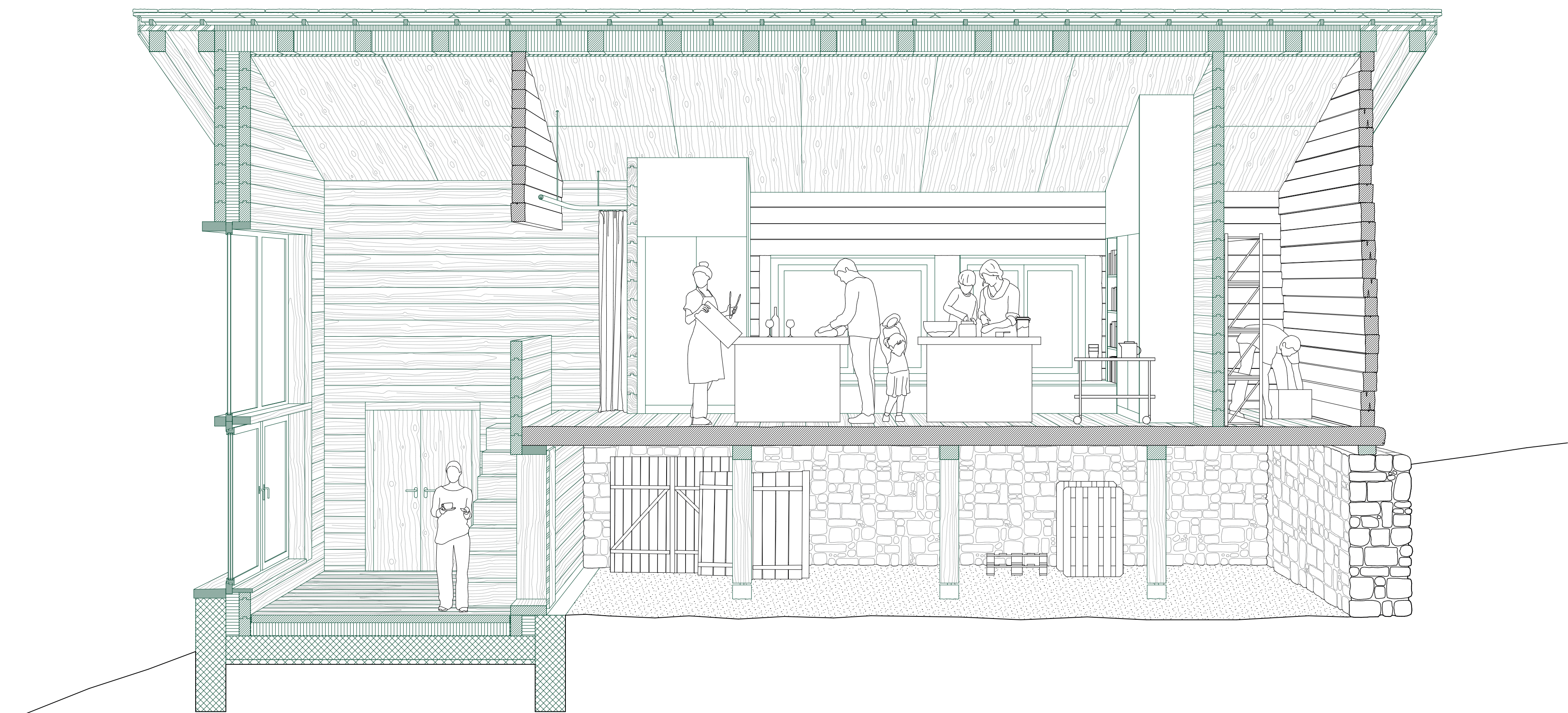
Section common kitchen 1:33
