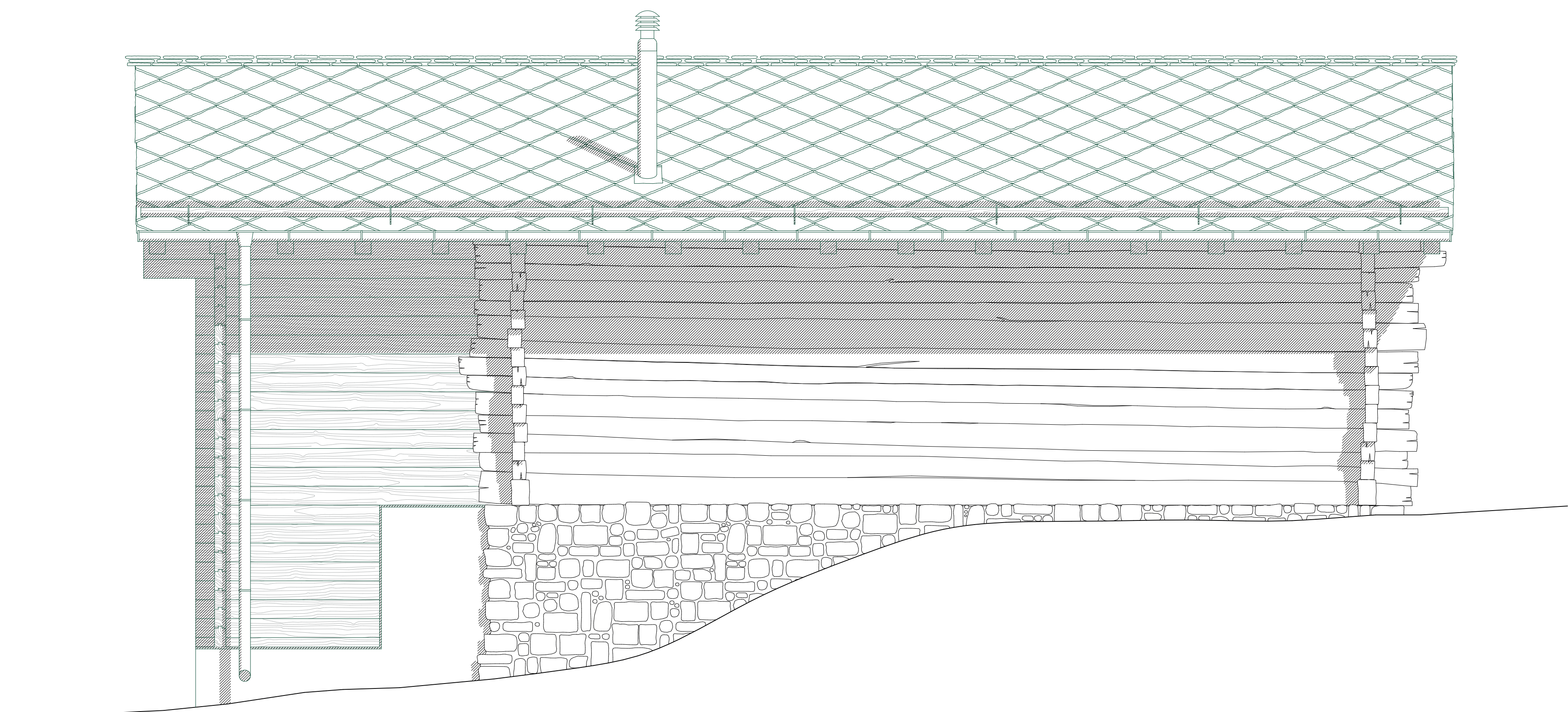
East facade common kitchen 1:33
