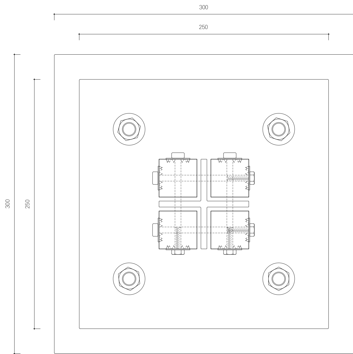
Plan Ancre
