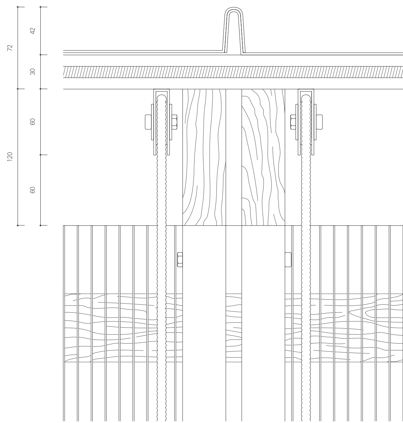
Elevation Façade
