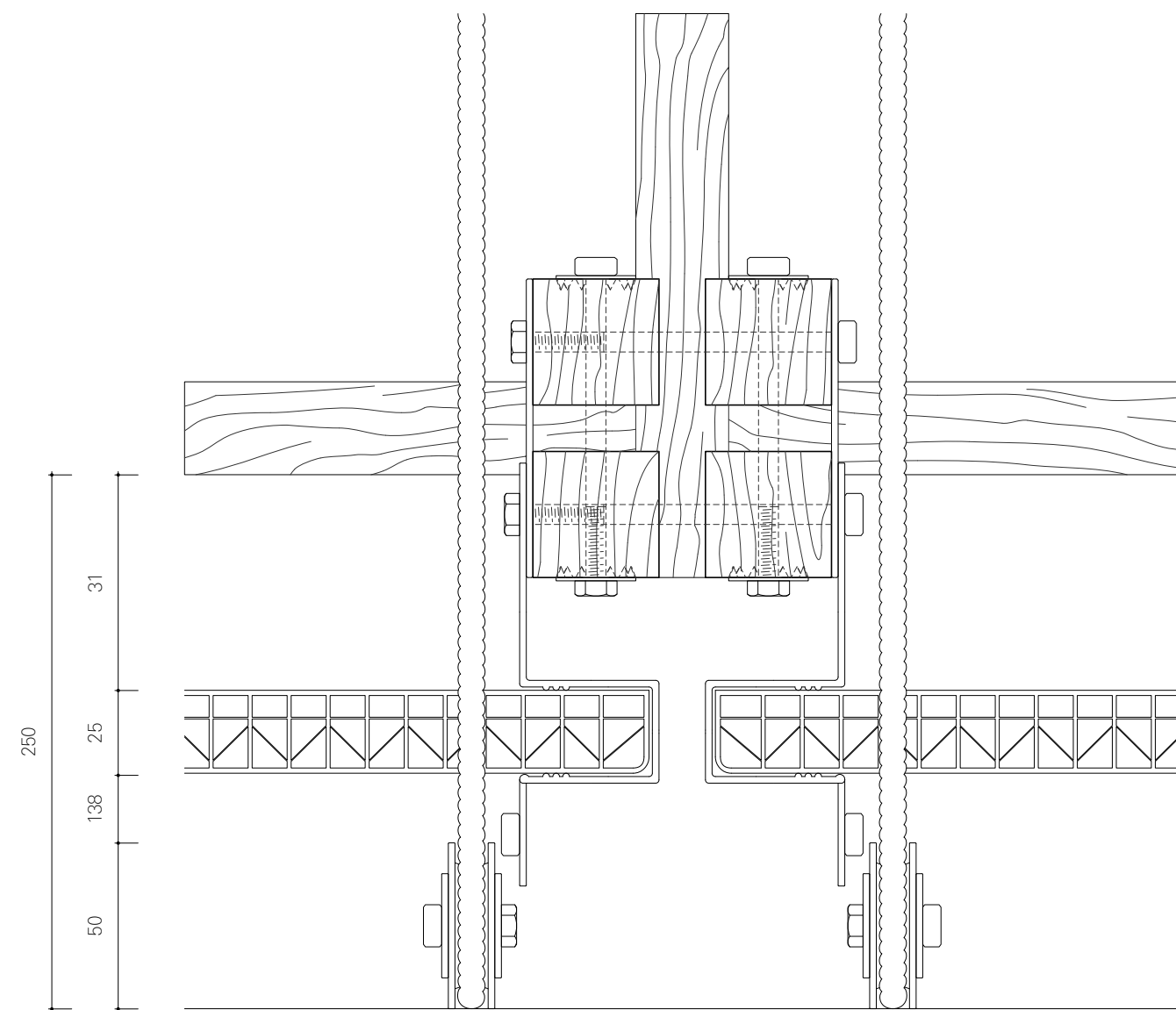
Plan Façade
