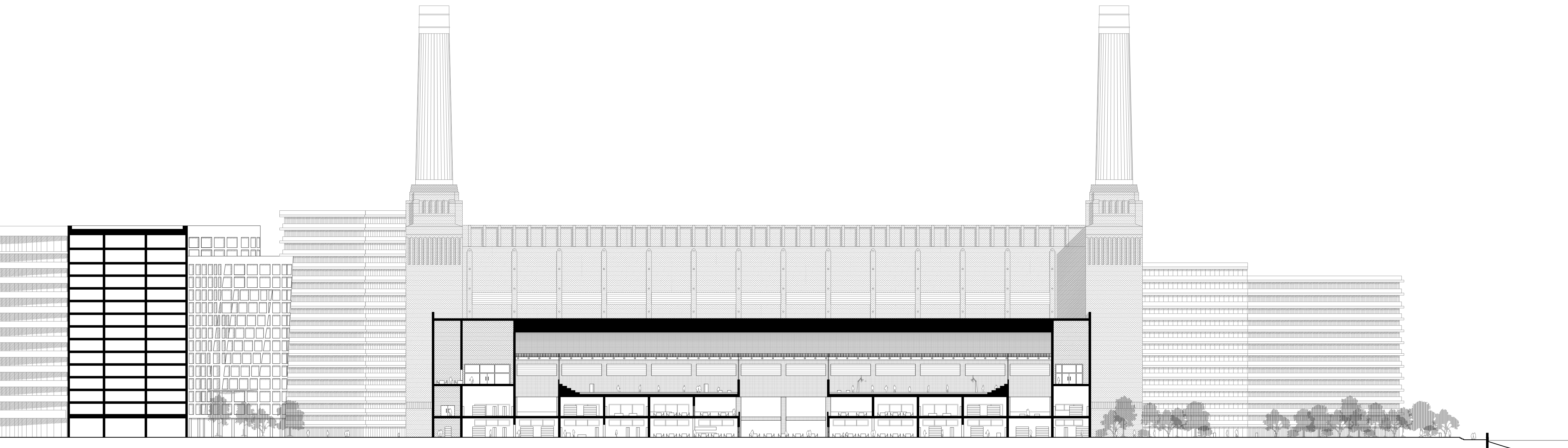
Section D-D' 1:500
