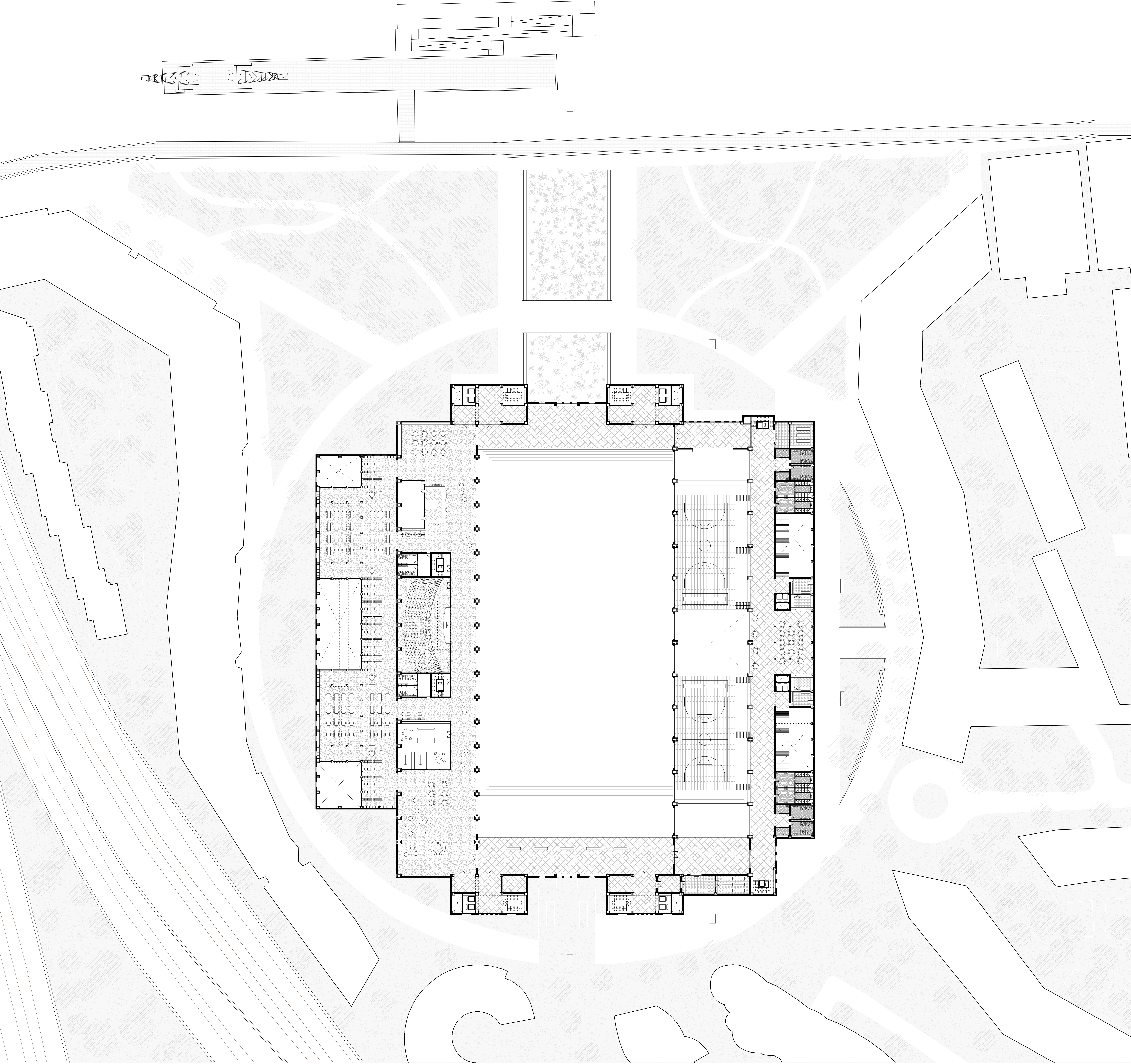
Second Floor 1:500
