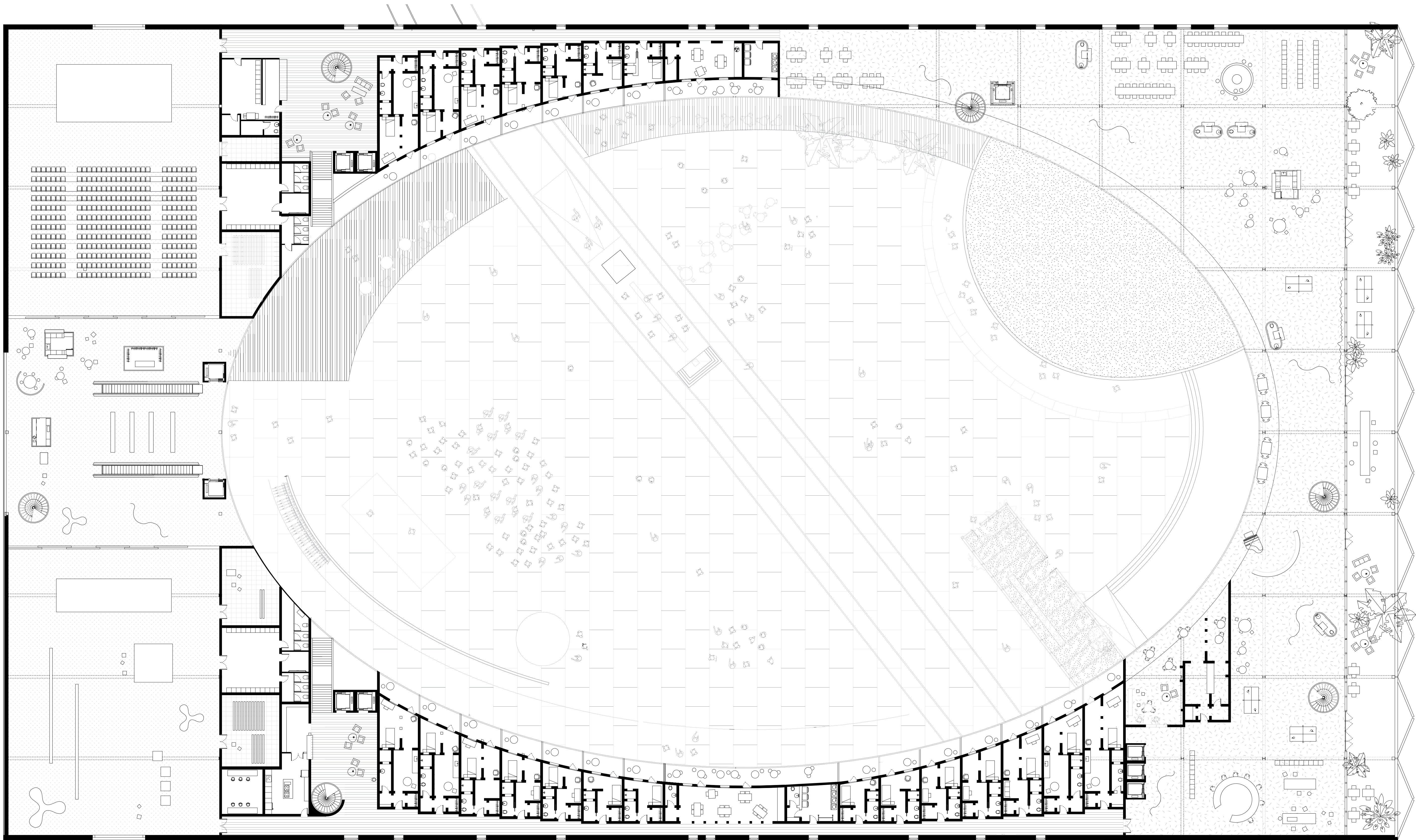
Plan +4.50
