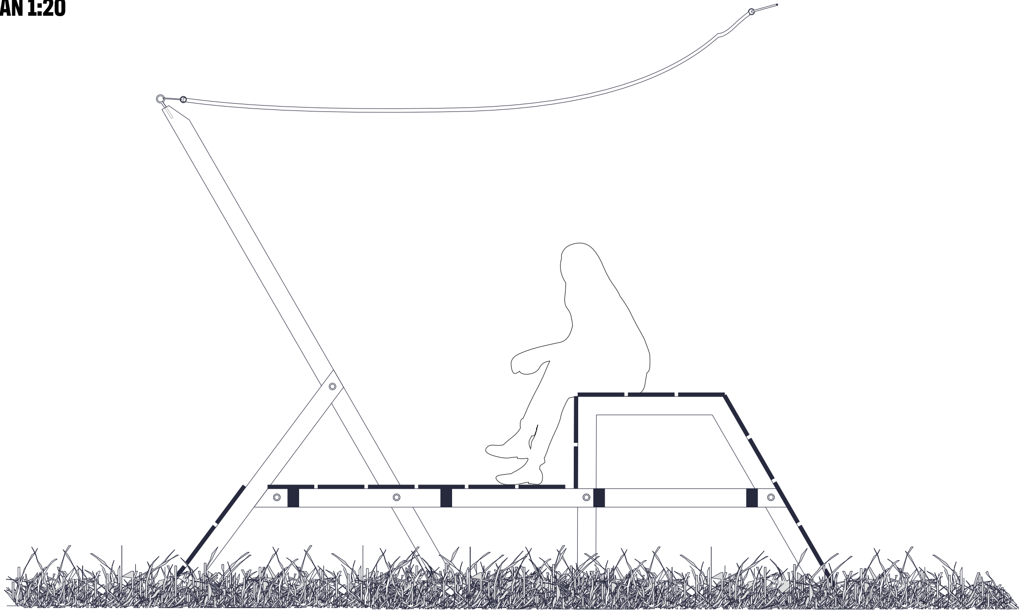
ASSISES "VOILE" PLAN 1:20
