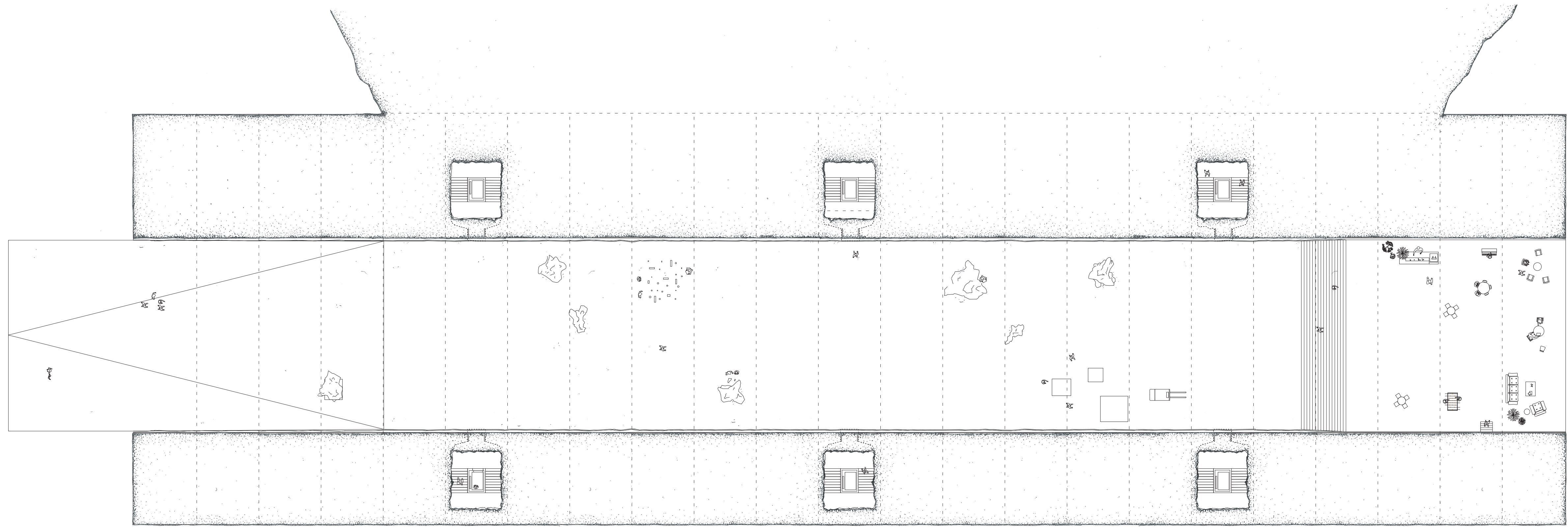
Plan foyer 1:250
