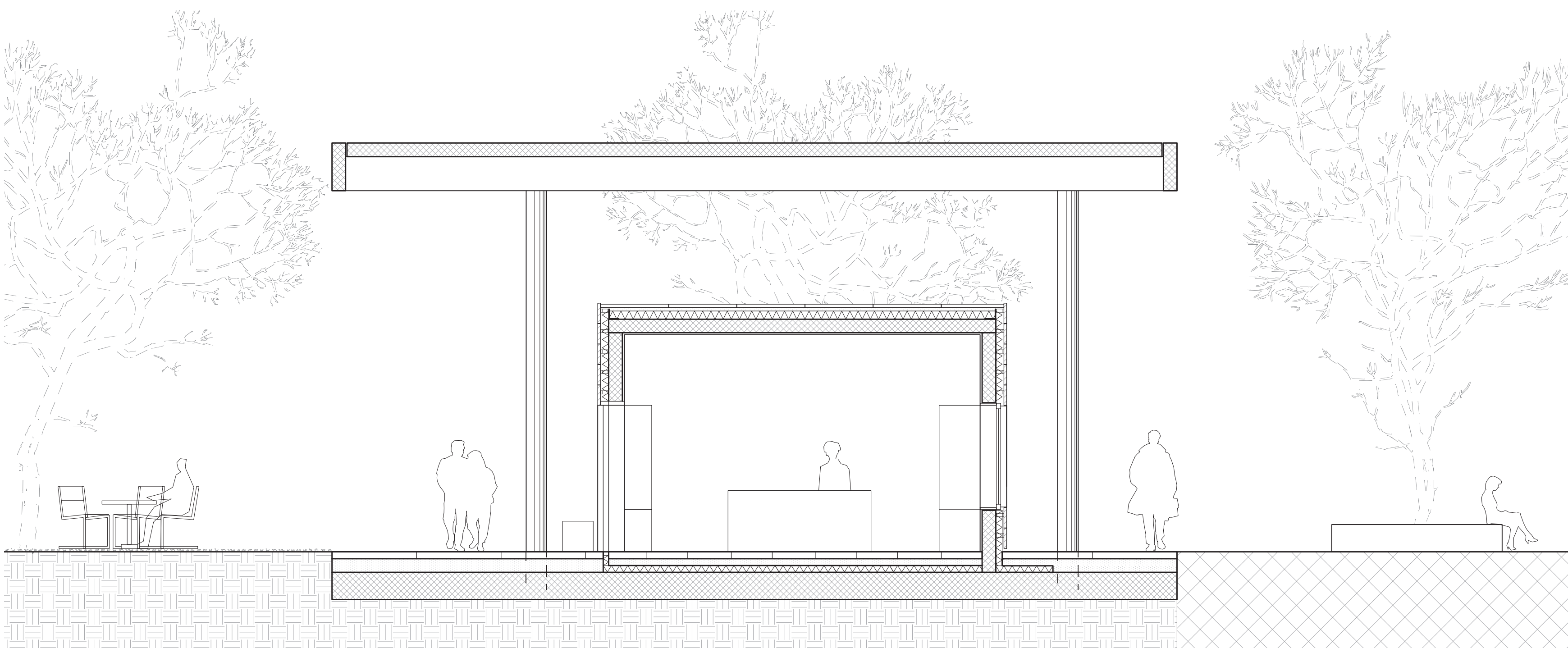
SECTION SHOP. SCALE 1/50
