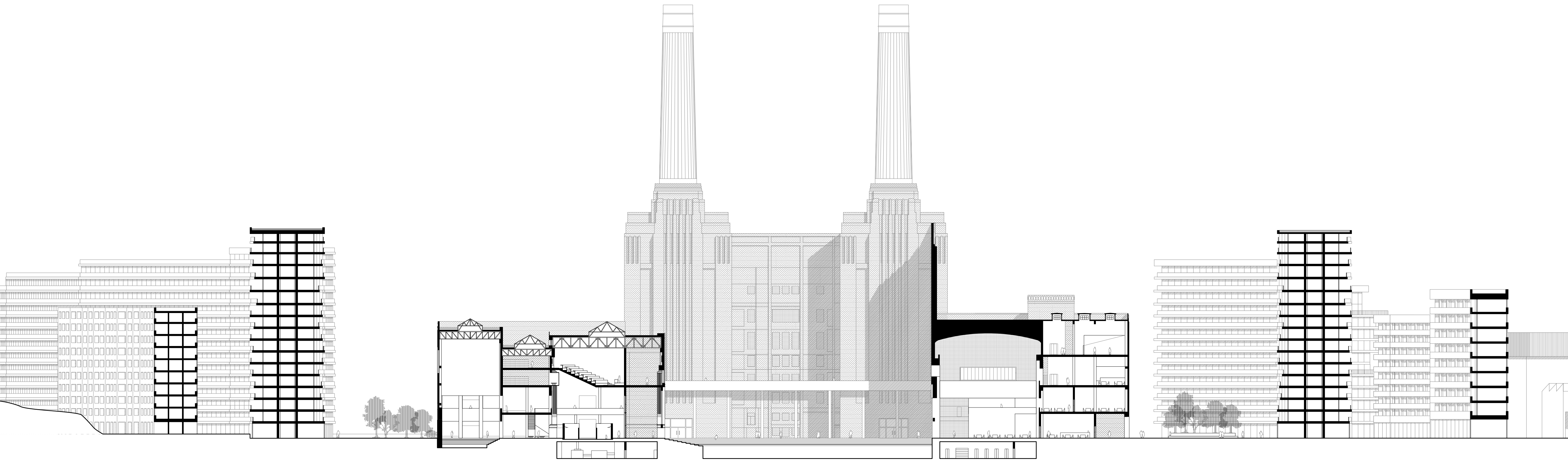
Section E-E 1: 500
