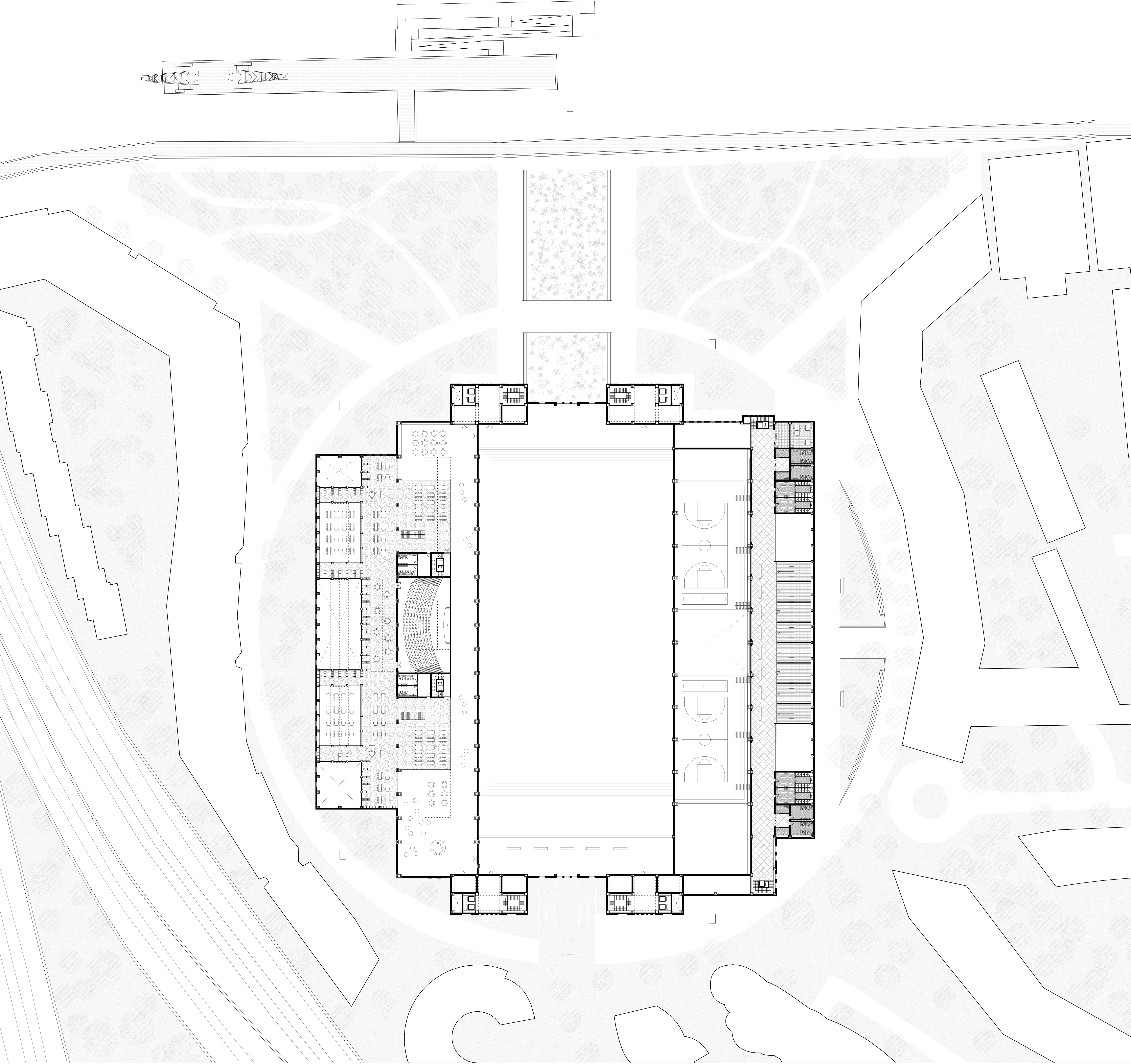
Third Floor 1:500
