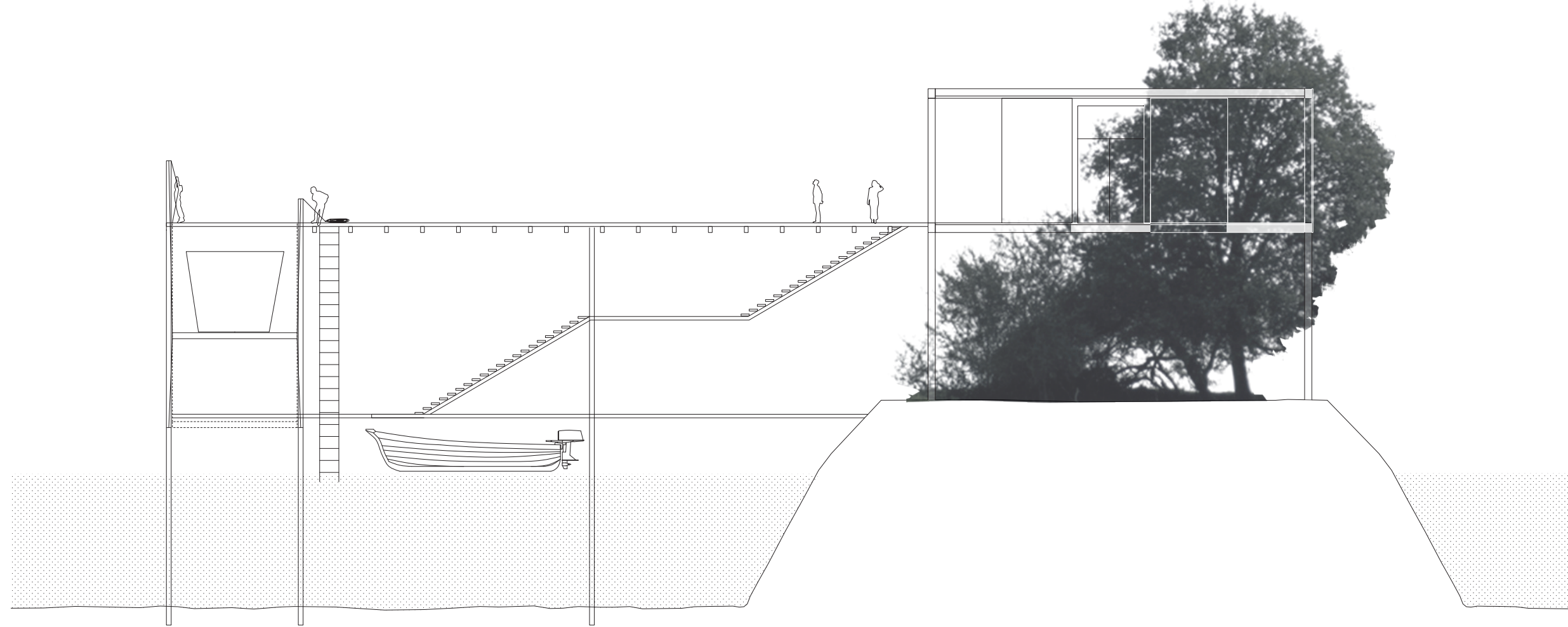
Section AA 1:200
