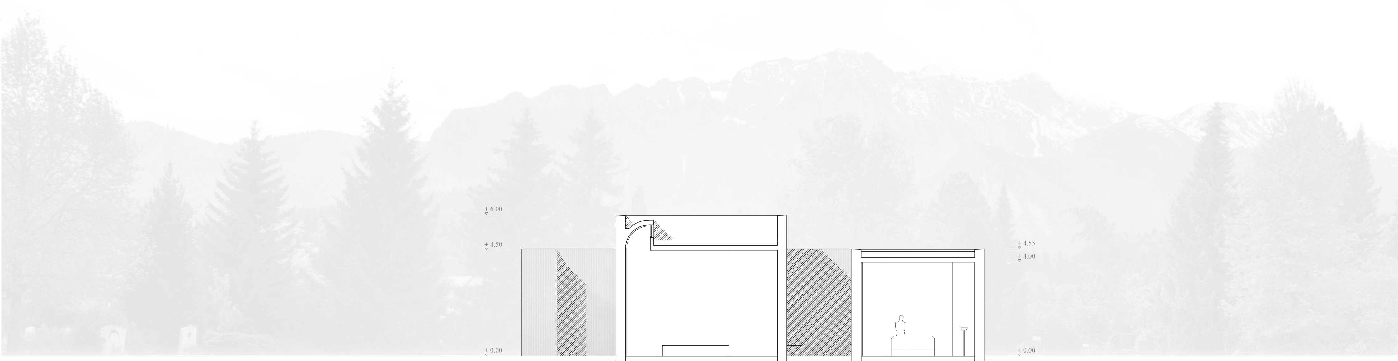
CROSS SECTION 1:100
