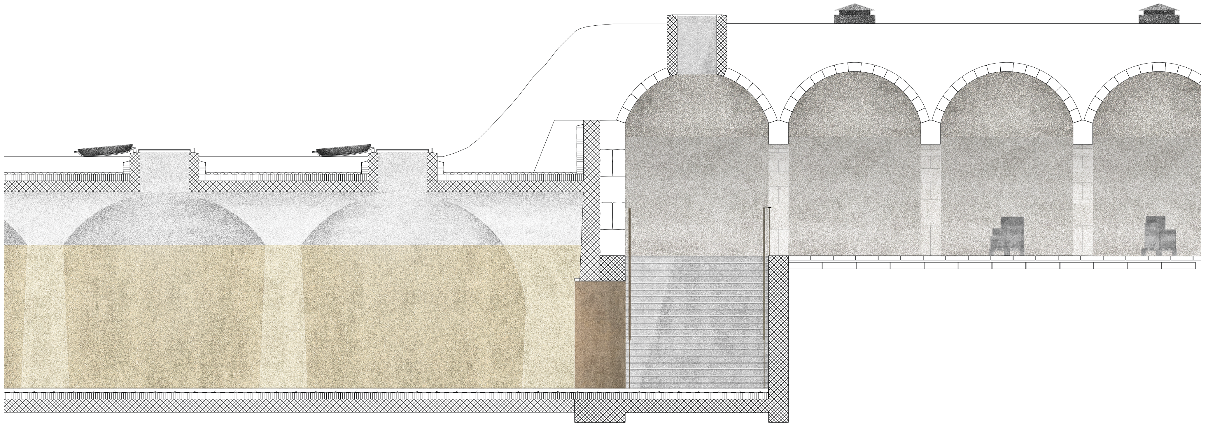
Detail \ Transition Filter III-Vorbassin \ 1:50
