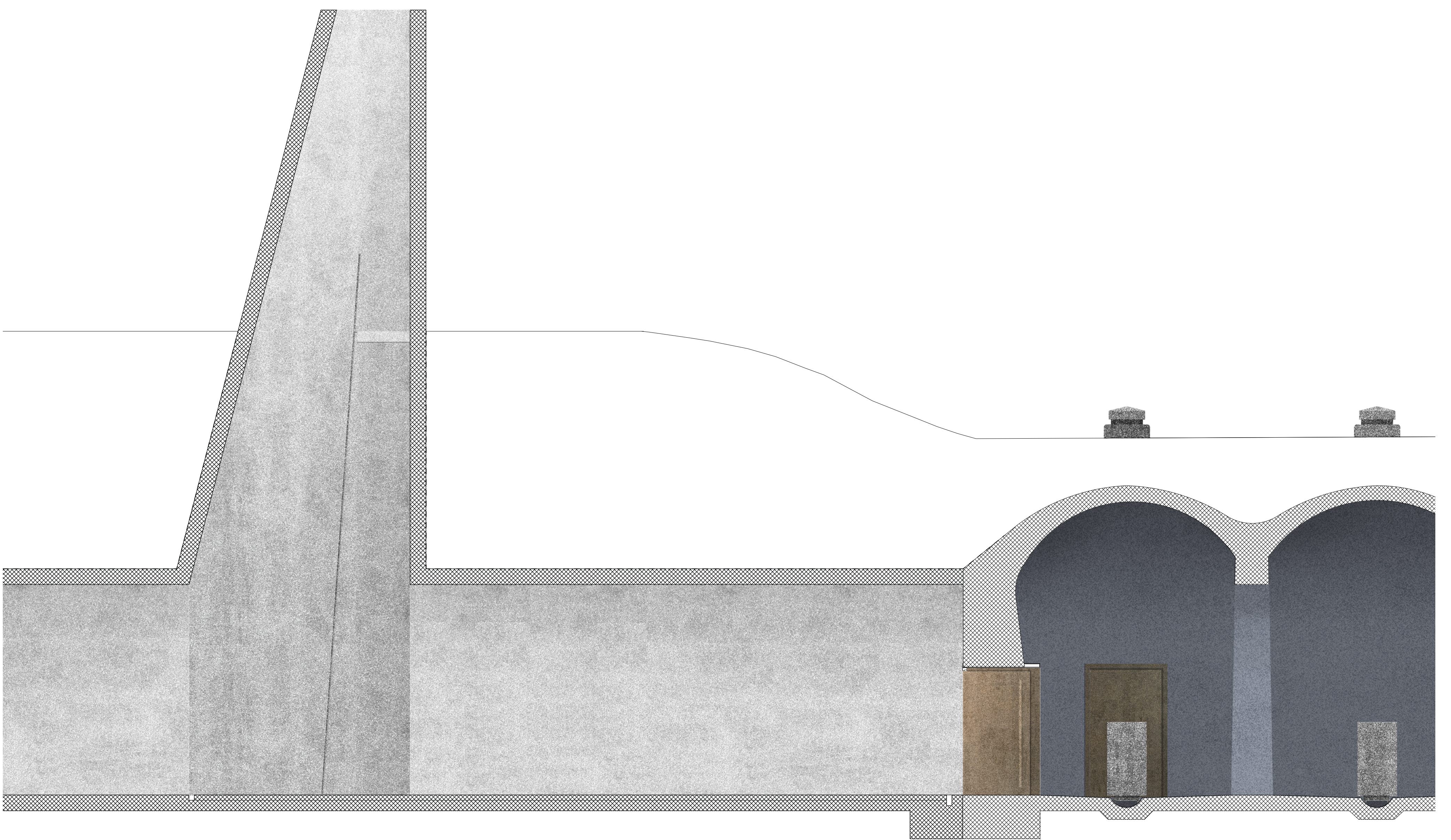
Detail \ Transition Light-schacht \ 1:50
