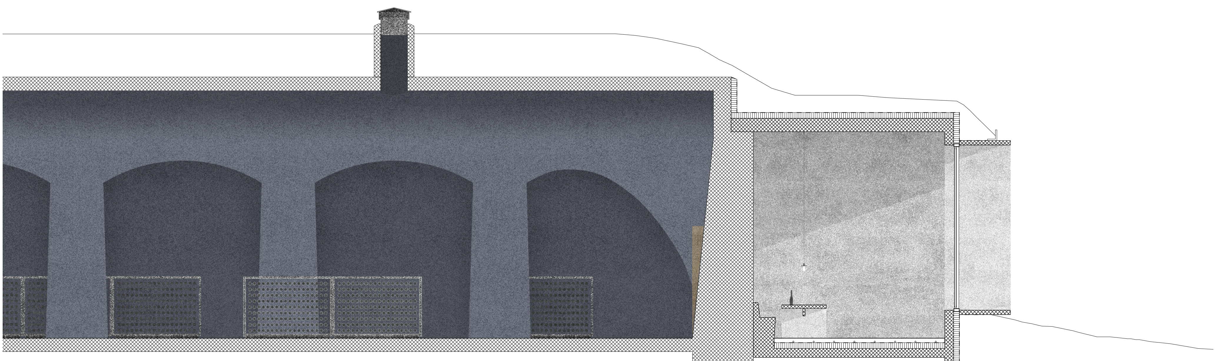
Detail \ The Tasting Room \ Reservoir \ 1:50
