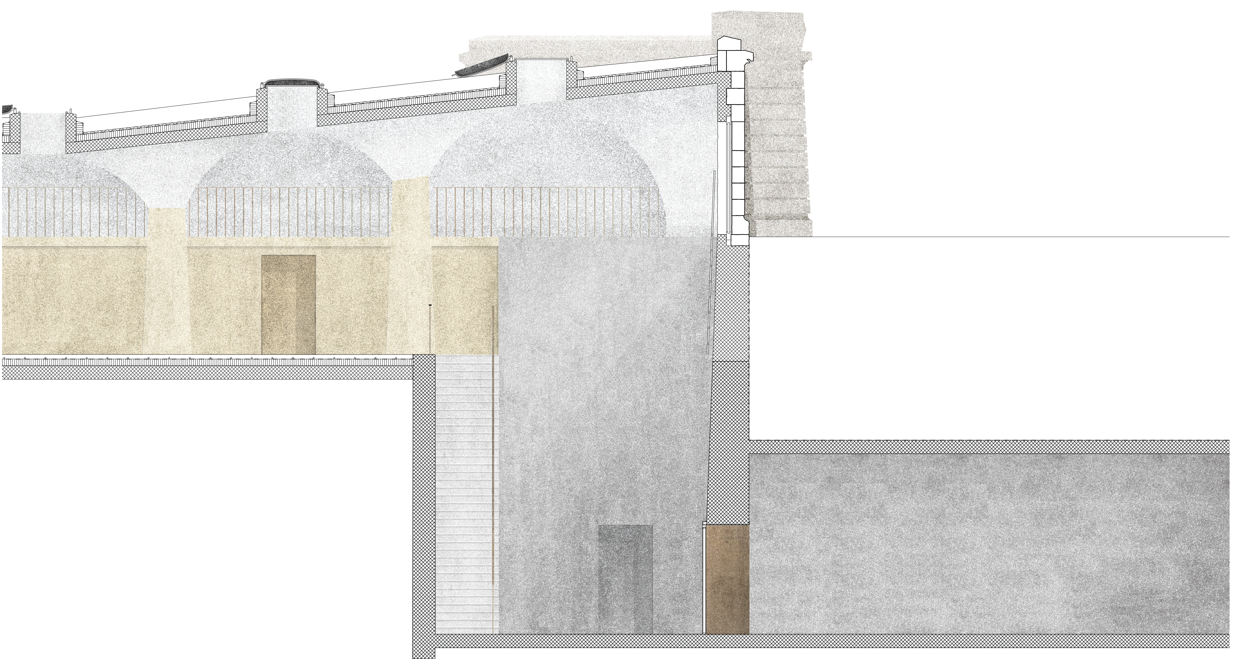
Detail \ Transition Filter II & Reservoir \ 1:50
