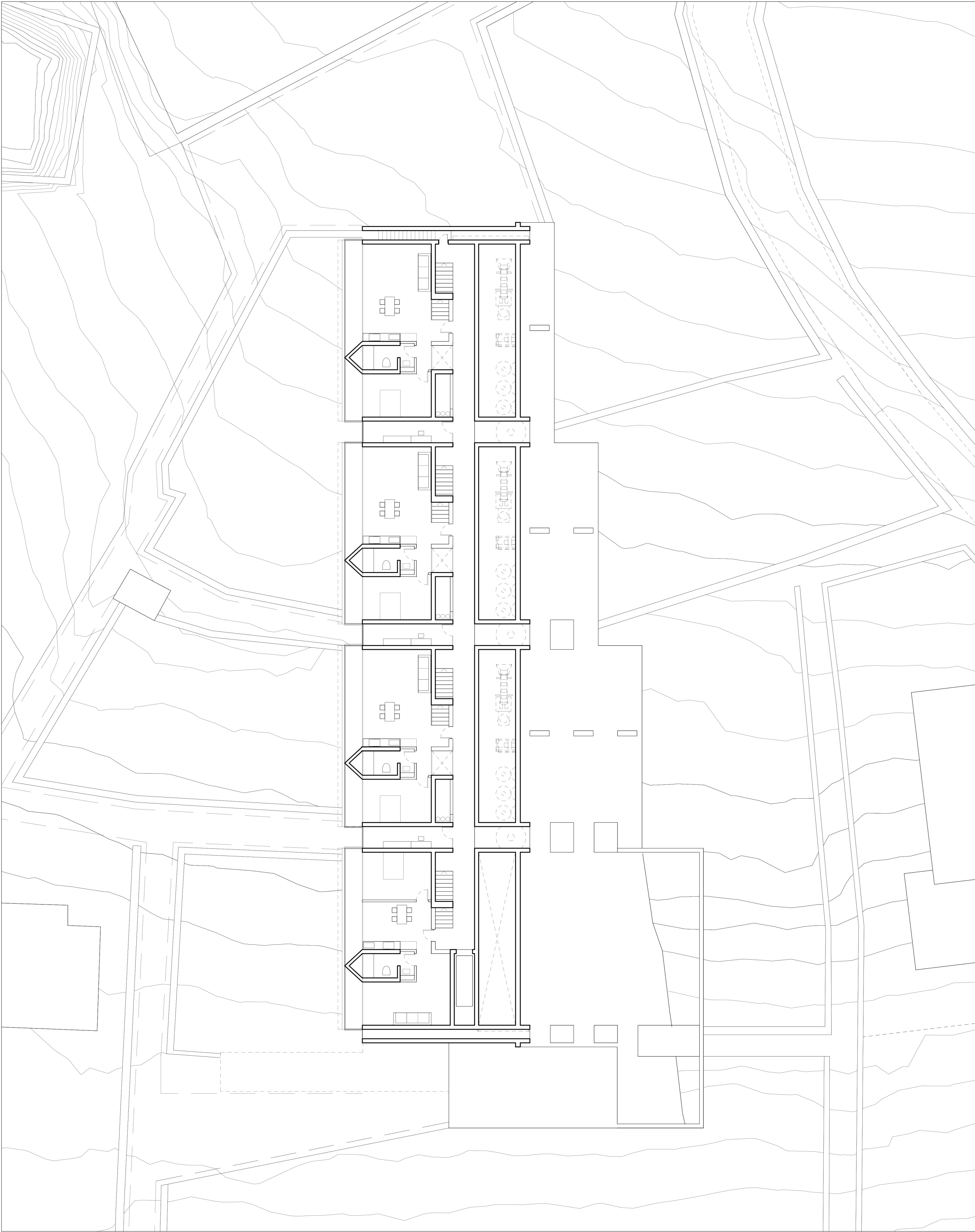
Plan +5.40m 1:200
