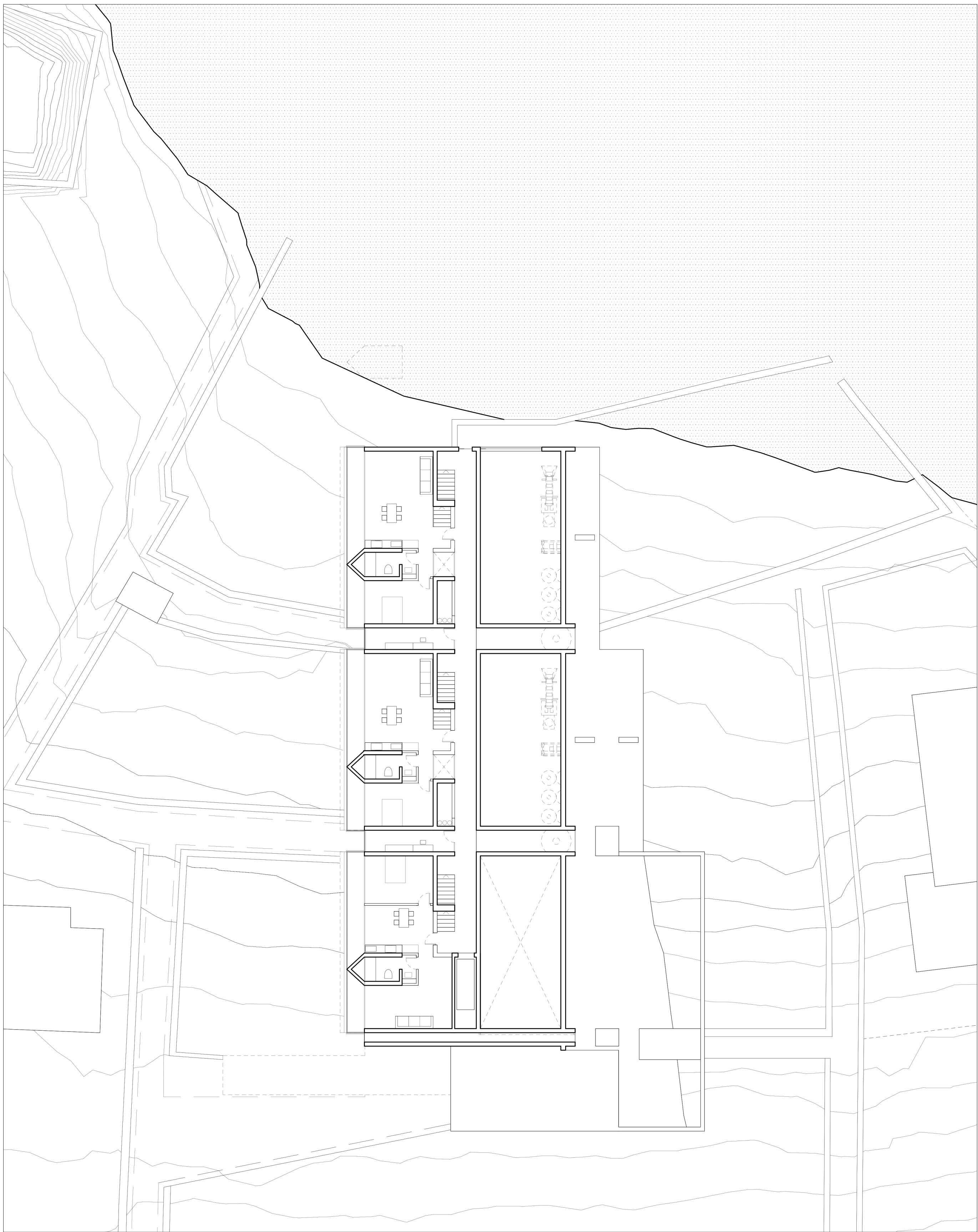
Plan - 2.70m 1:200
