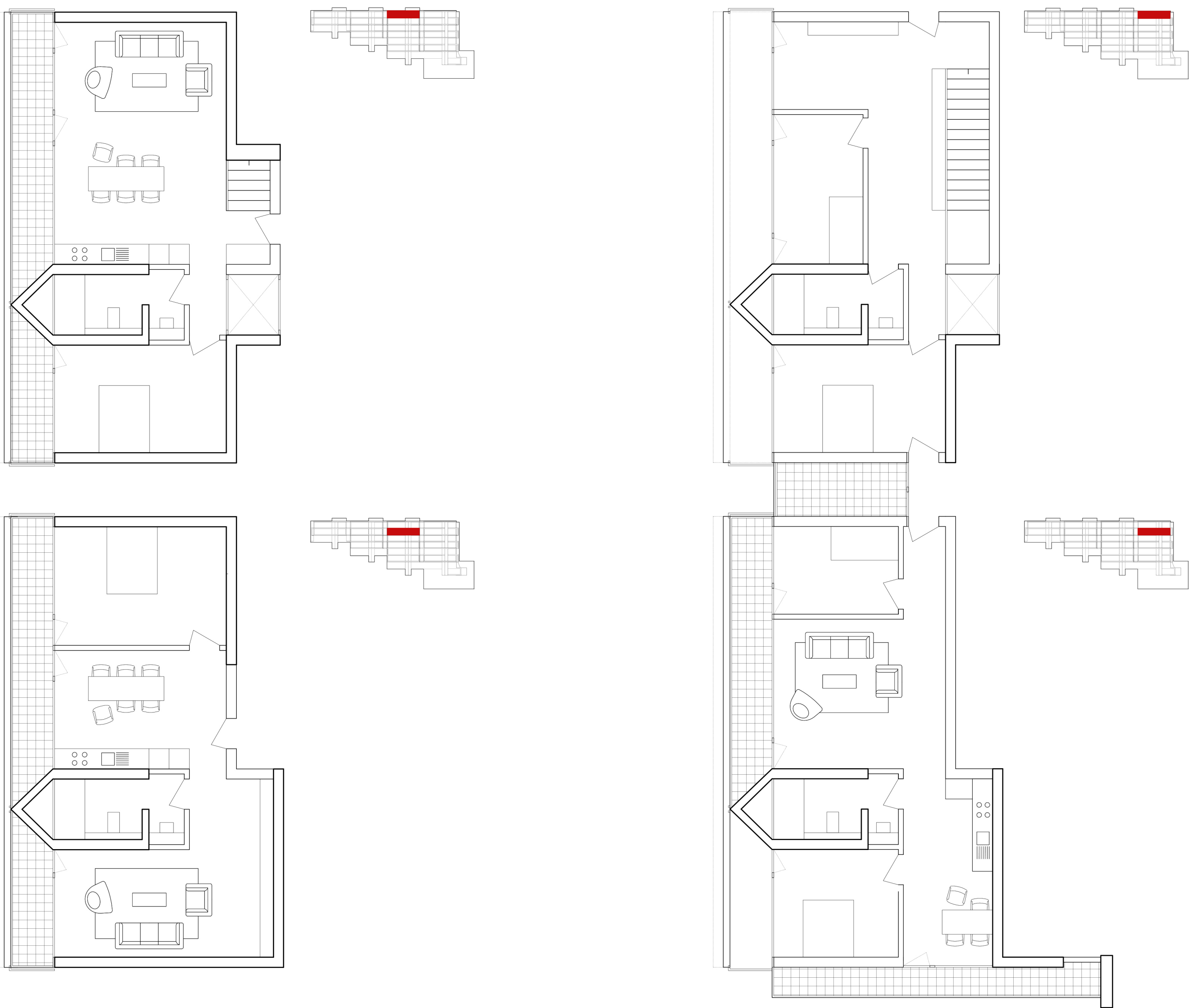
Plan - 5.40m 1:200
