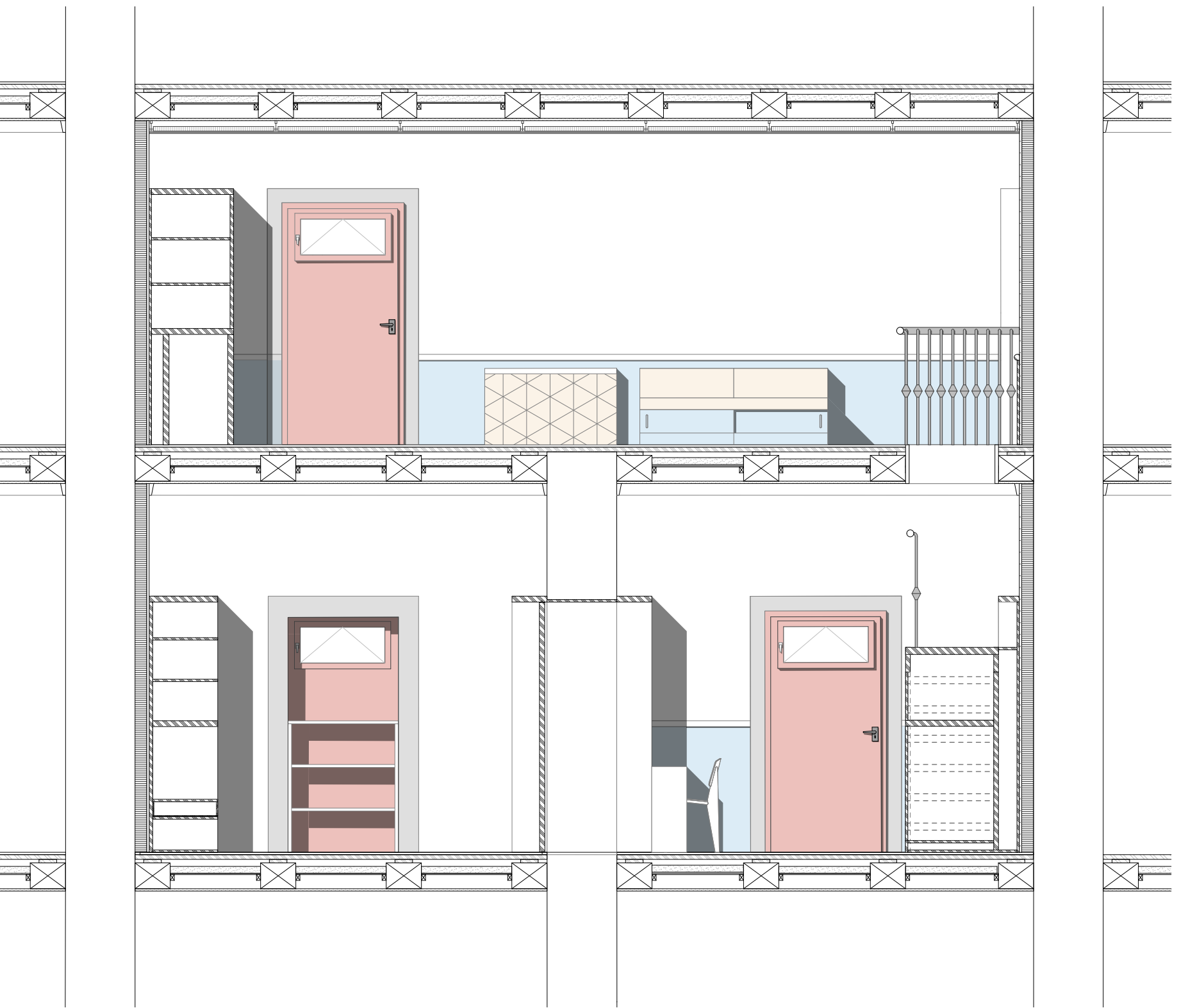
Coupe K'-K
