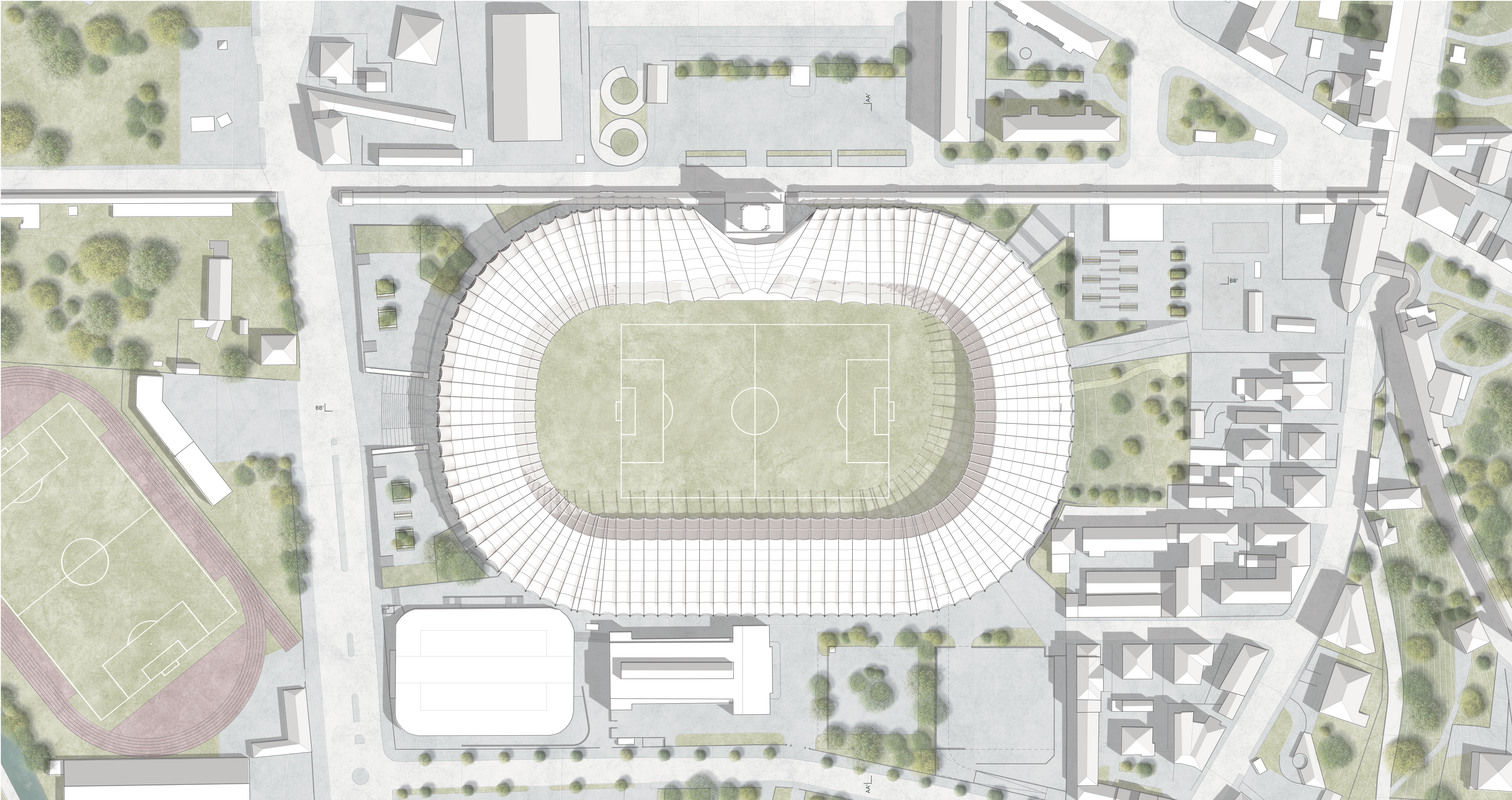
Situation 1:500
