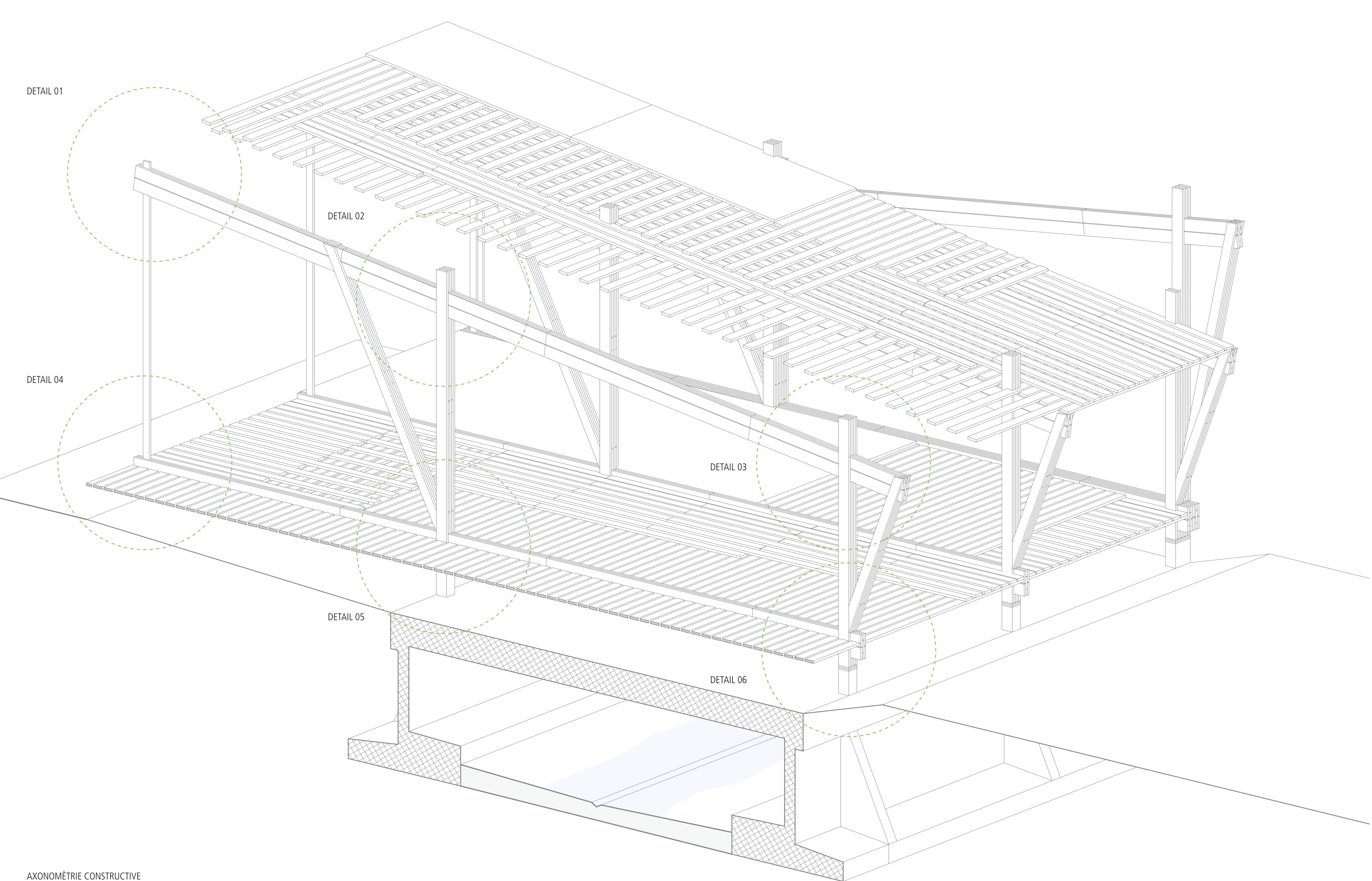
AXONOMETRIE CONSTRUCTIVE
