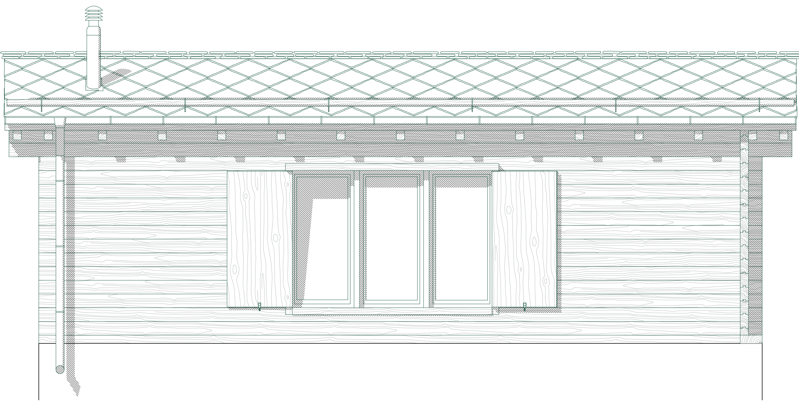
South facade common room 1:33
