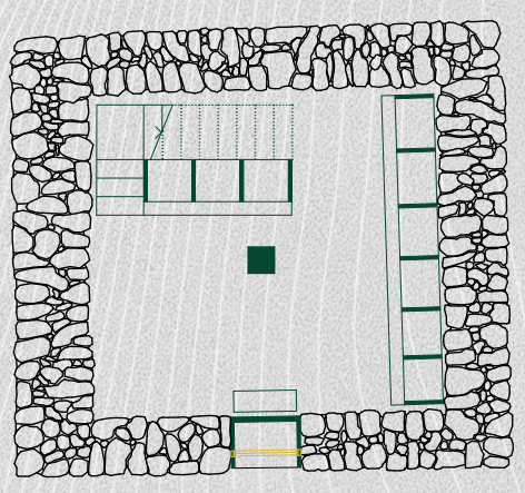
Lower floor plan local shop 1:100
