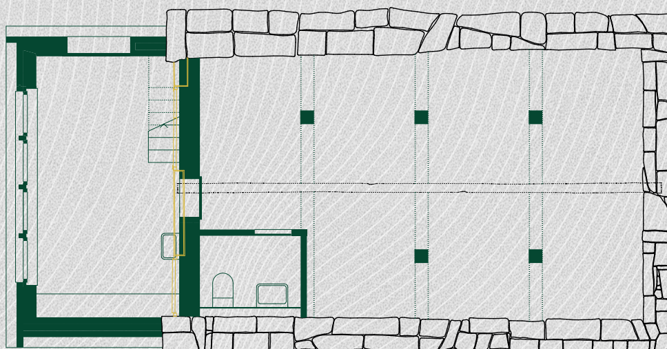
Lower floor plan common kitchen 1:100
