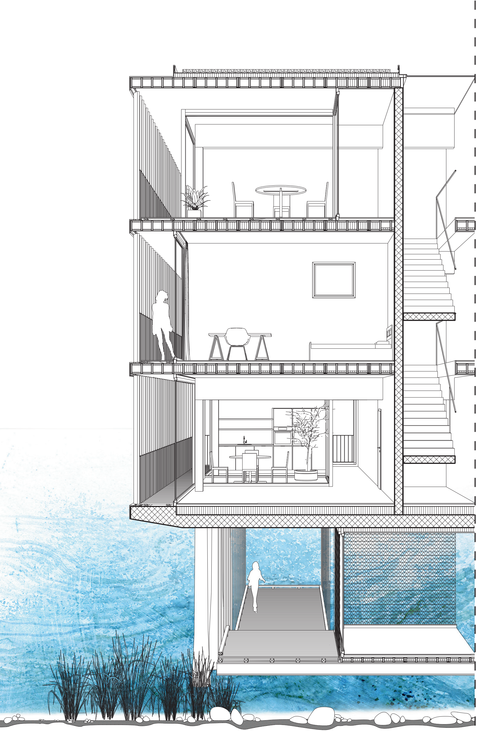
DETAILS 1:50
