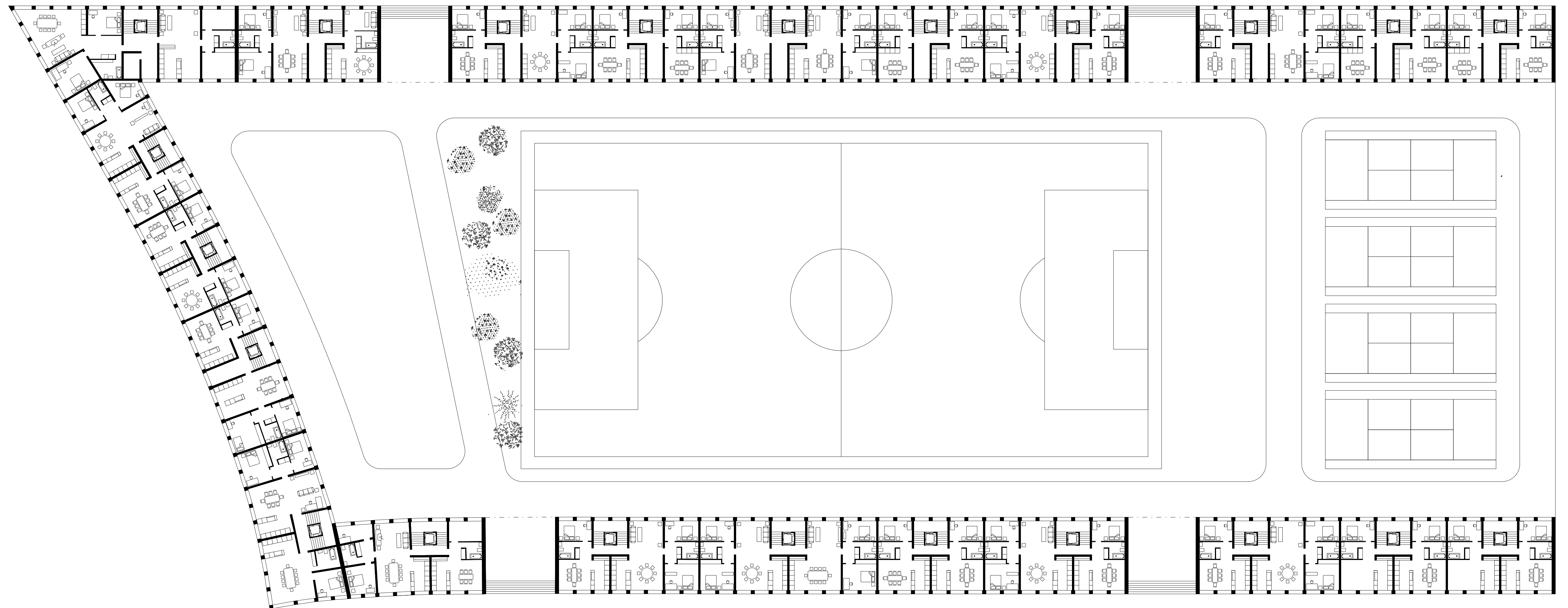
Groundfloor
