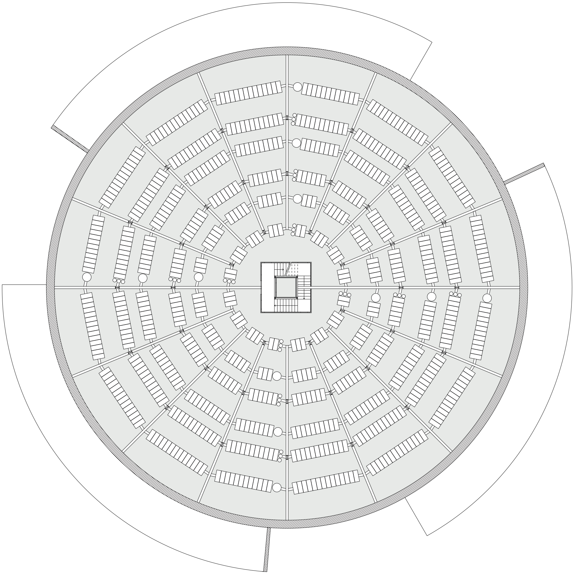
SERVER LEVEL PLAN - 1:200
