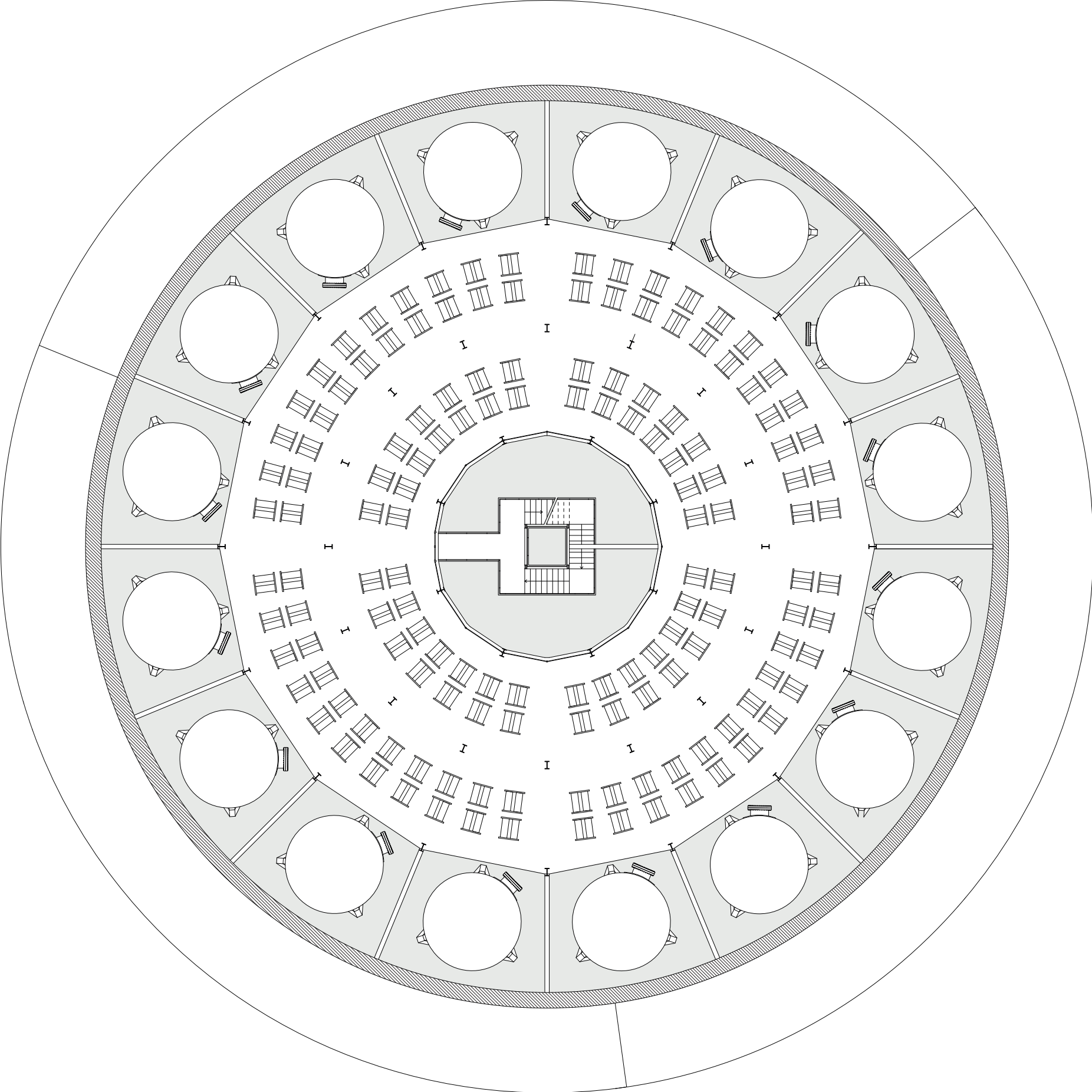
HYDROGEN STORAGE LEVEL PLAN - 1:200
