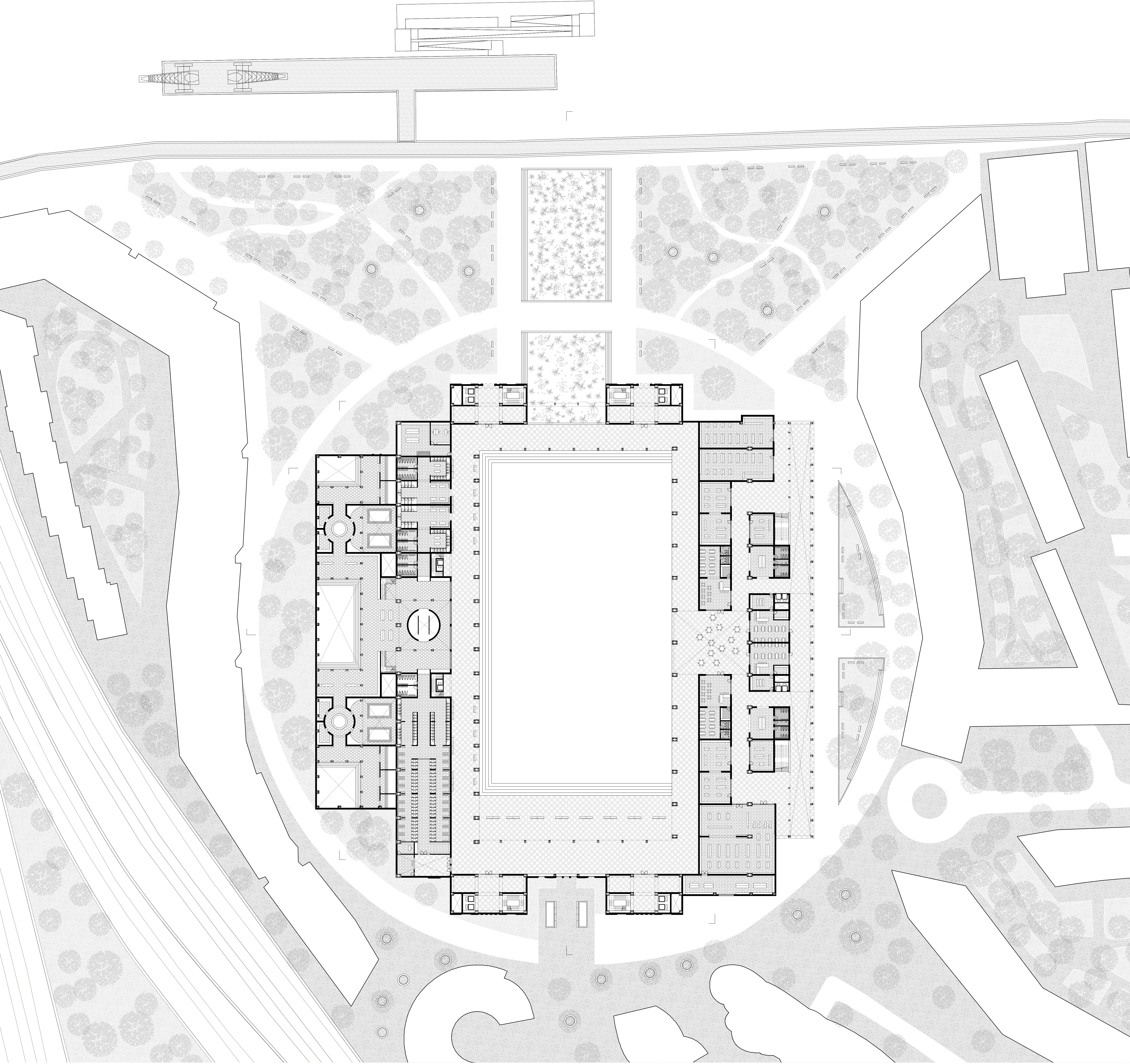
Ground Floor 1:500
