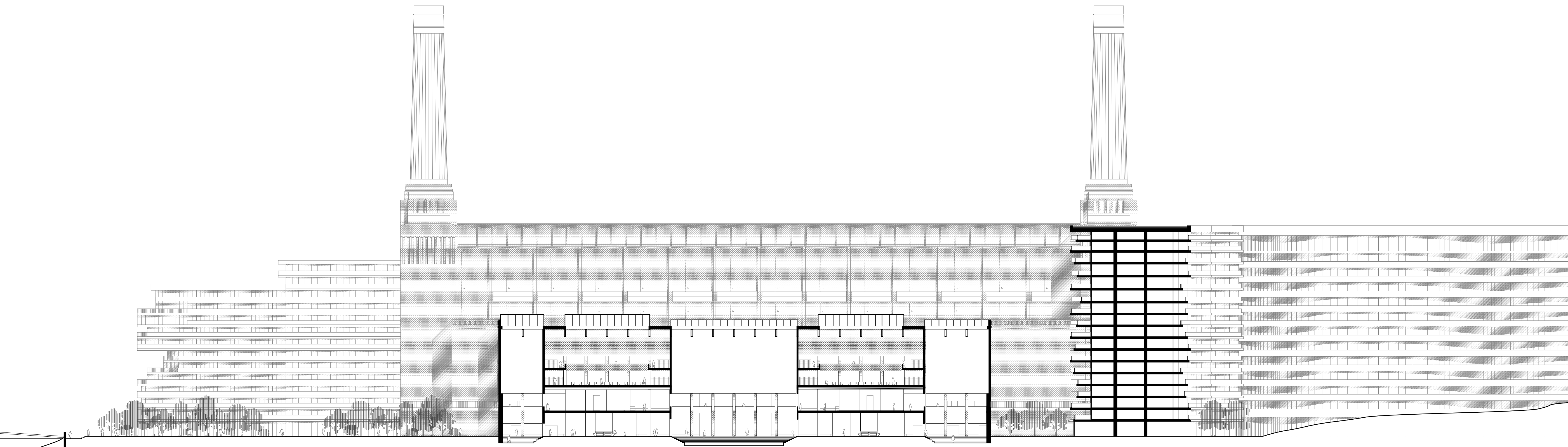
Section B-B 1: 500
