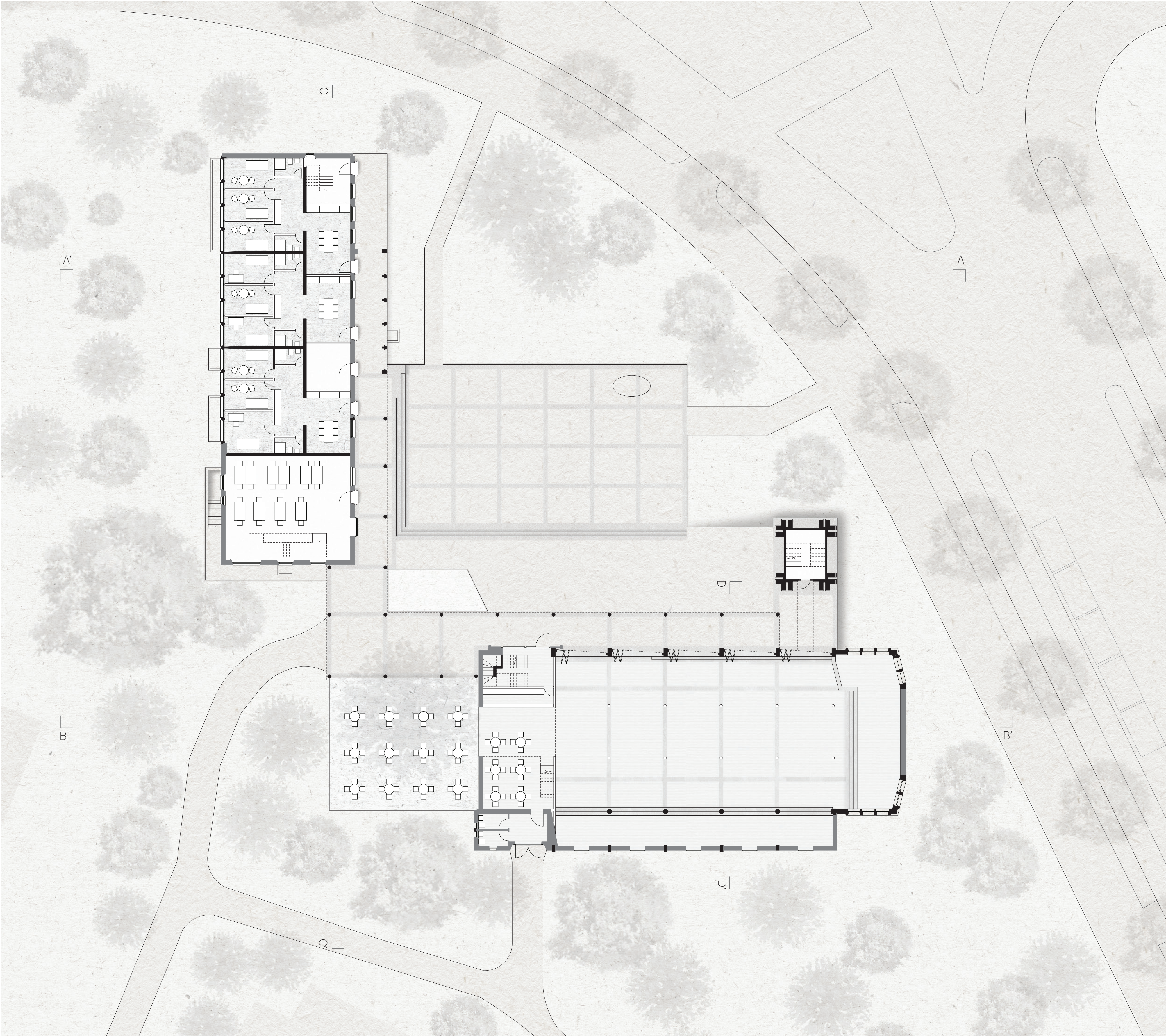
Plan rez 1:200
