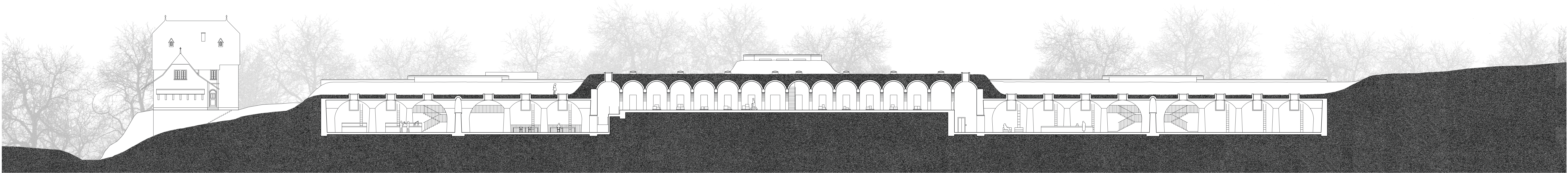
Section BB' | 1:200
