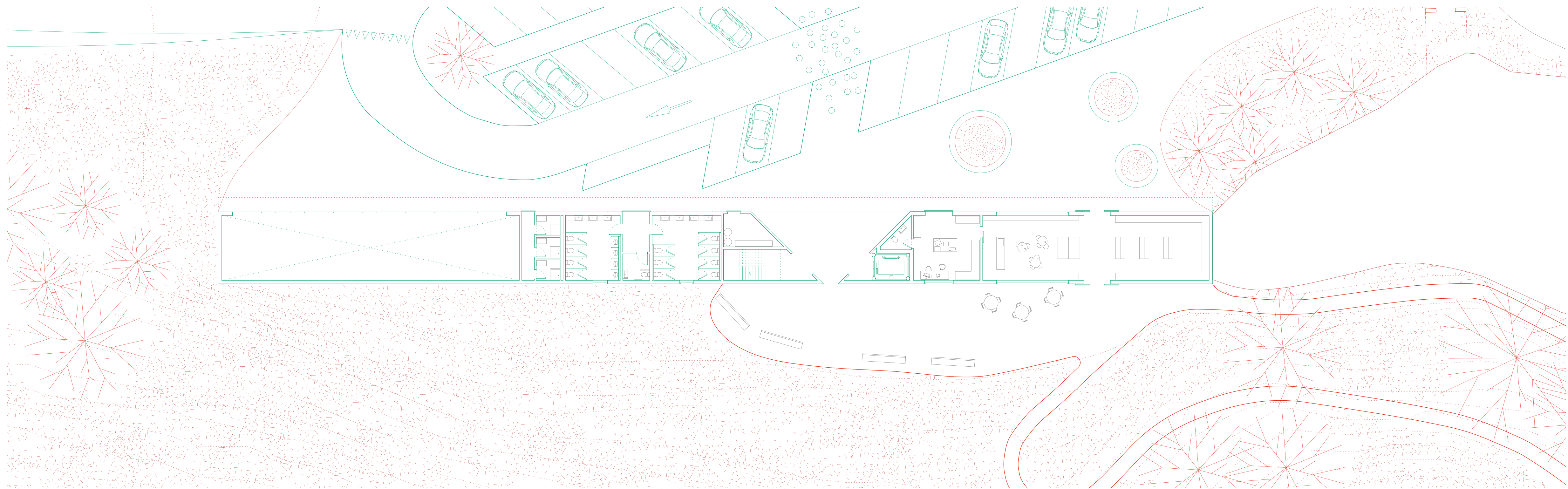
1: 200 Plan rez-de-chaussée, Station-service direction Vevey.
