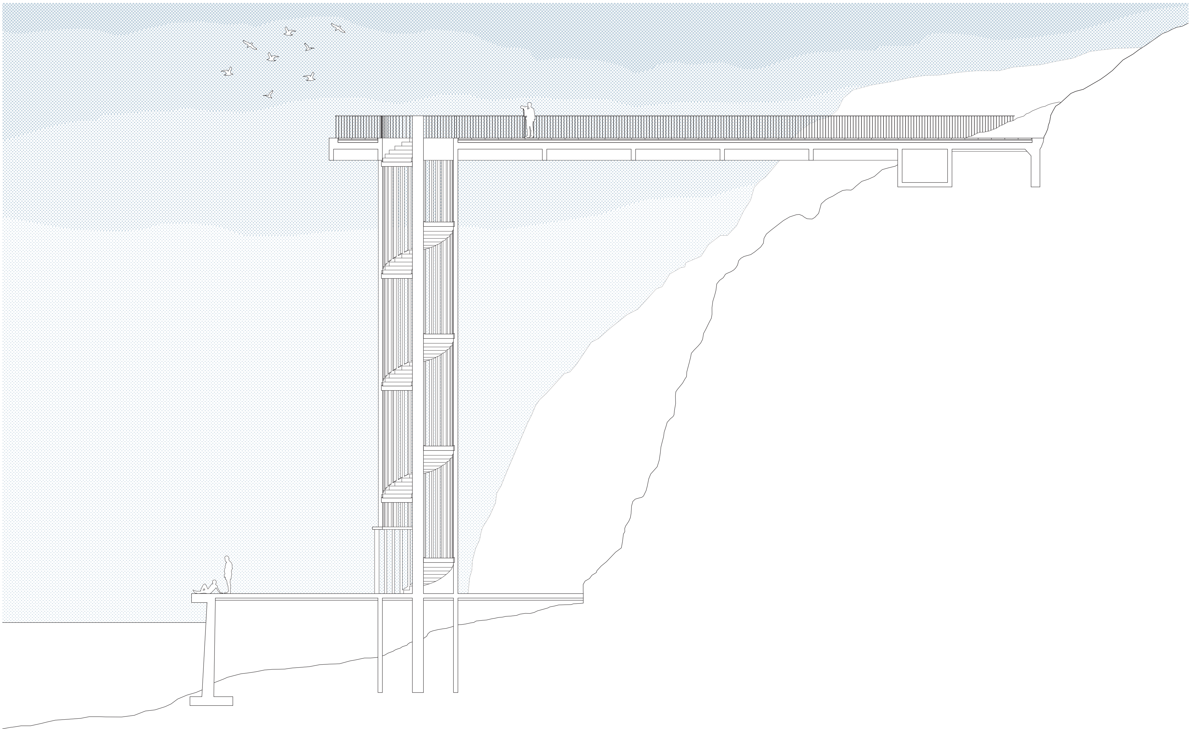
prototype #1: garipce - observation tower section 1:100
