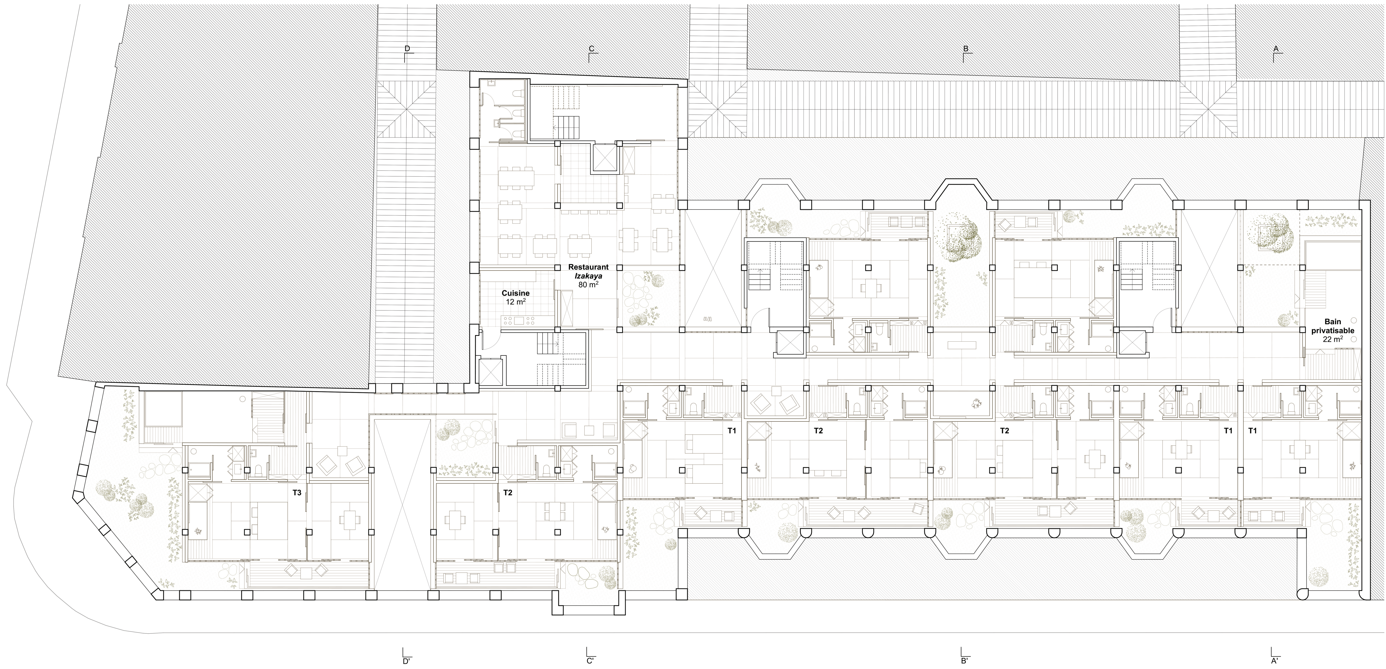
🕒 Etage 2, Plan Type 1/100e
