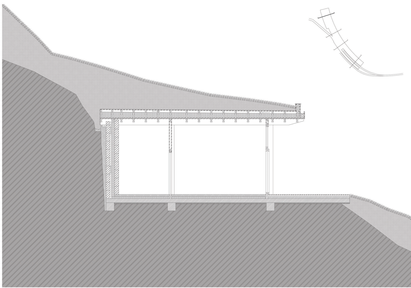
Section D 1.00 - Rochers de Naye Terminus Station
