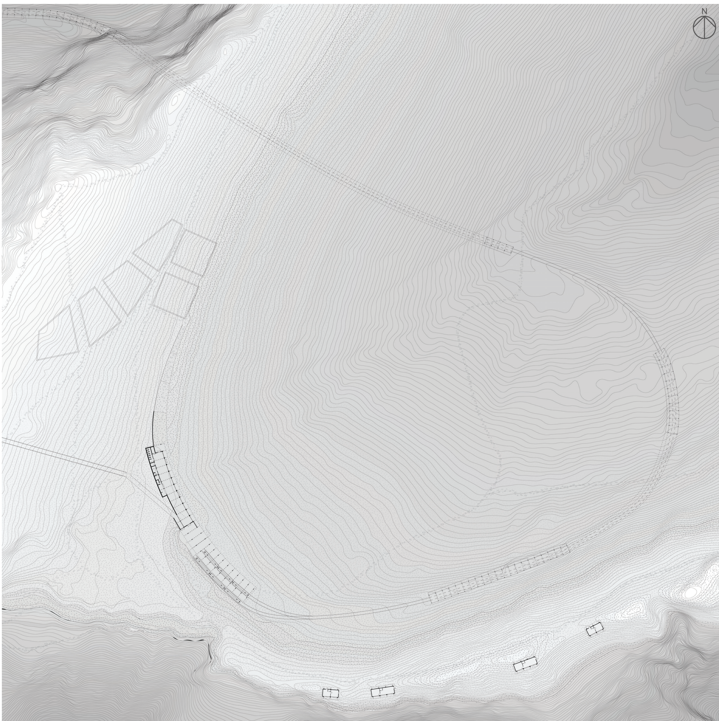
Mass plan 1:1250
