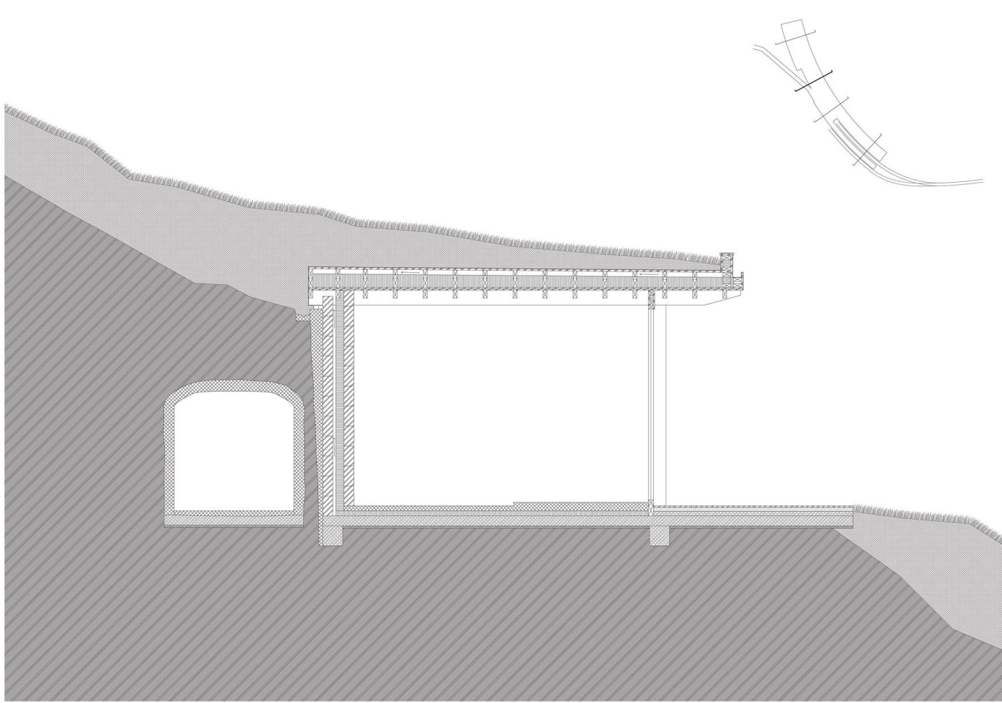
Section C 1.00 - Rochers de Naye Terminus Station
