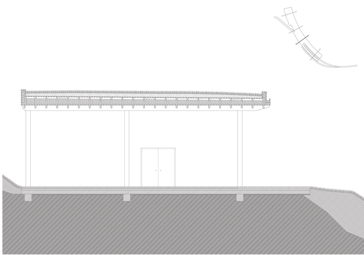
Section B 1.00 - Rochers de Naye Terminus Station
