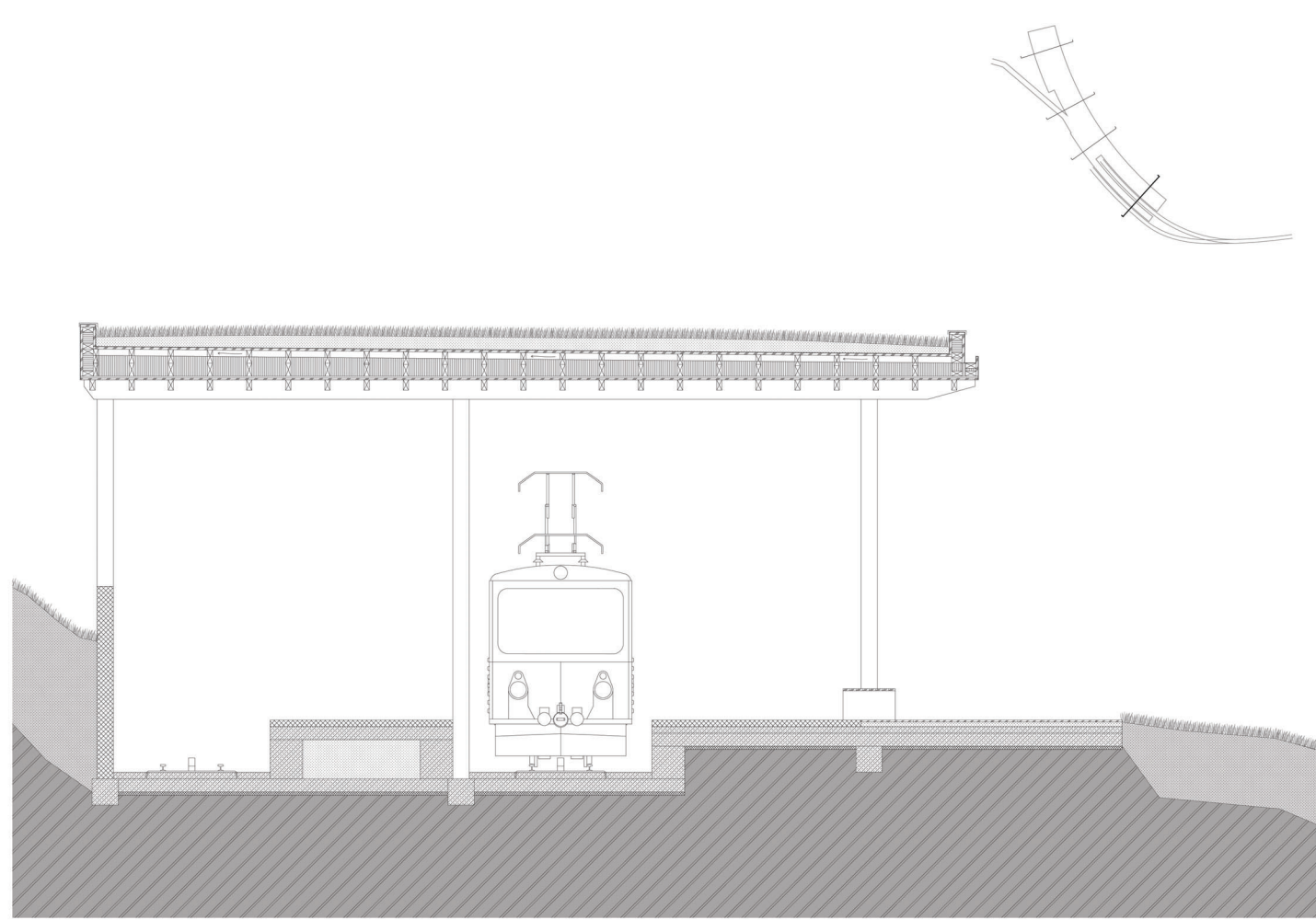
Section A 1.00 - Rochers de Naye Terminus Station
