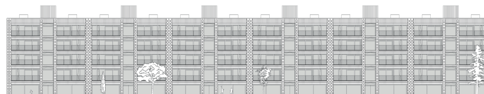
ELEVATIONS BATIMENT COTE FRONT URBAIN 1:200, BAS: FACADE INTERIEURE ILOT COMMUNAUTAIRE, HAUT: FACADE FRONT URBAIN
