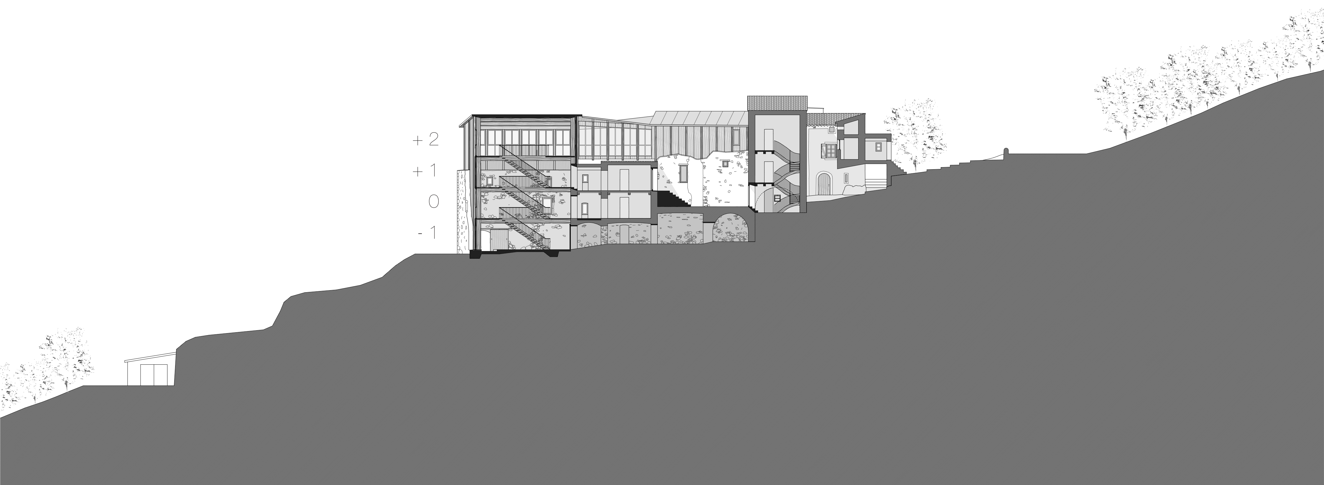
SECTION AA | 1:200
