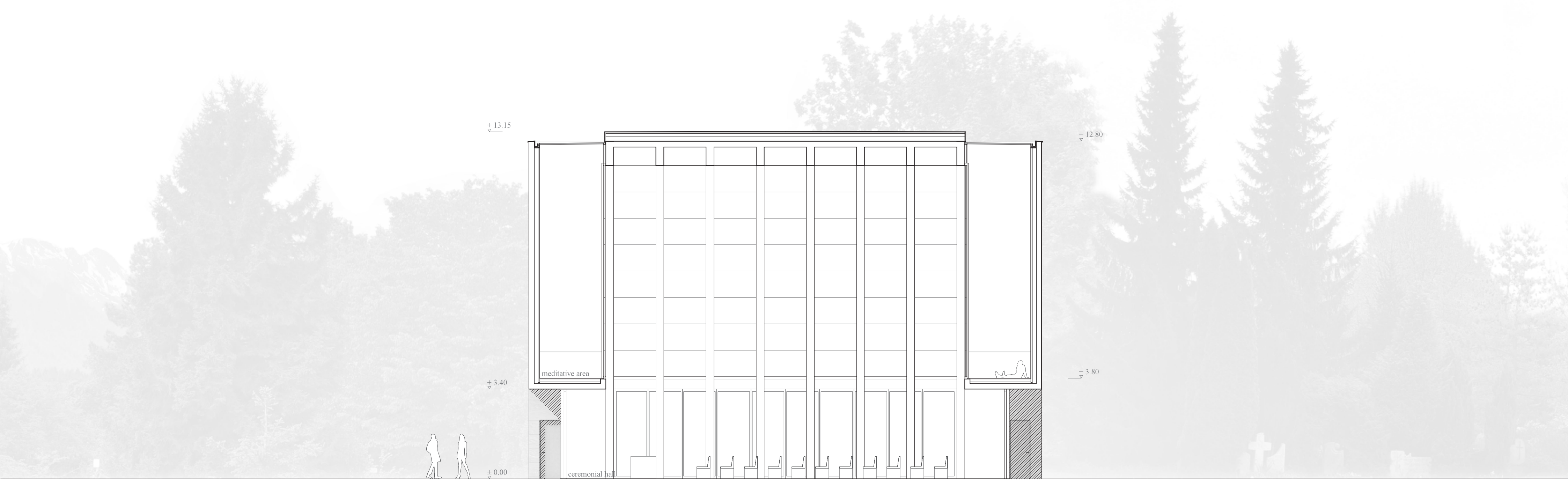
EAST-WEST SECTION 1:100
