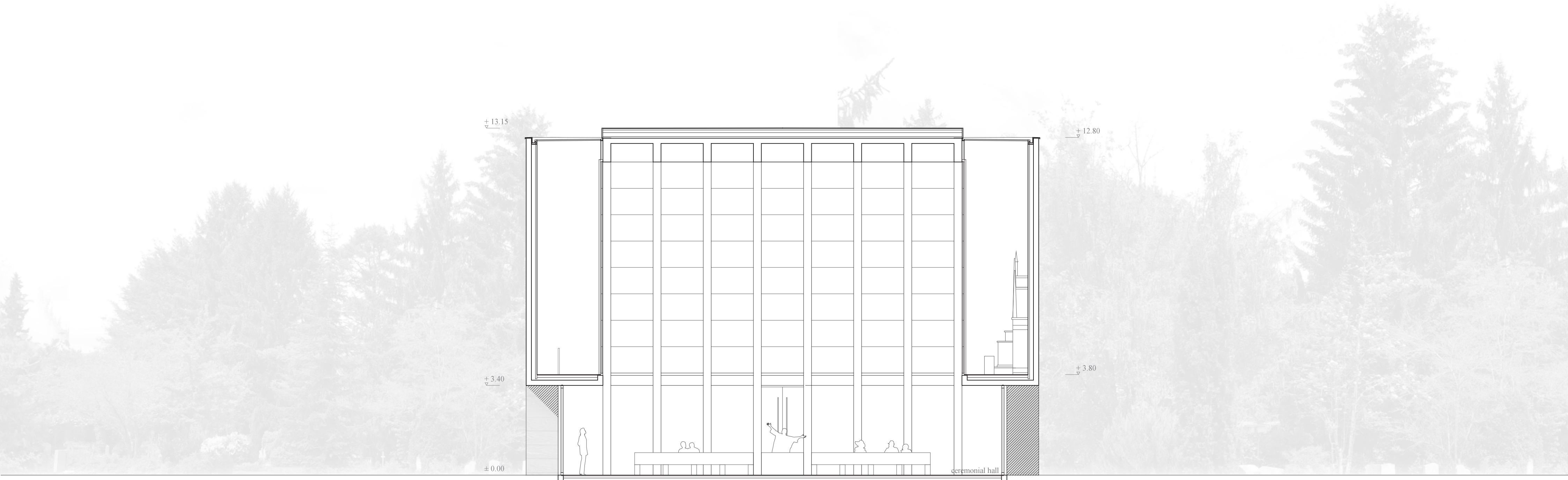
NORTH-SOUTH SECTION 1:100
