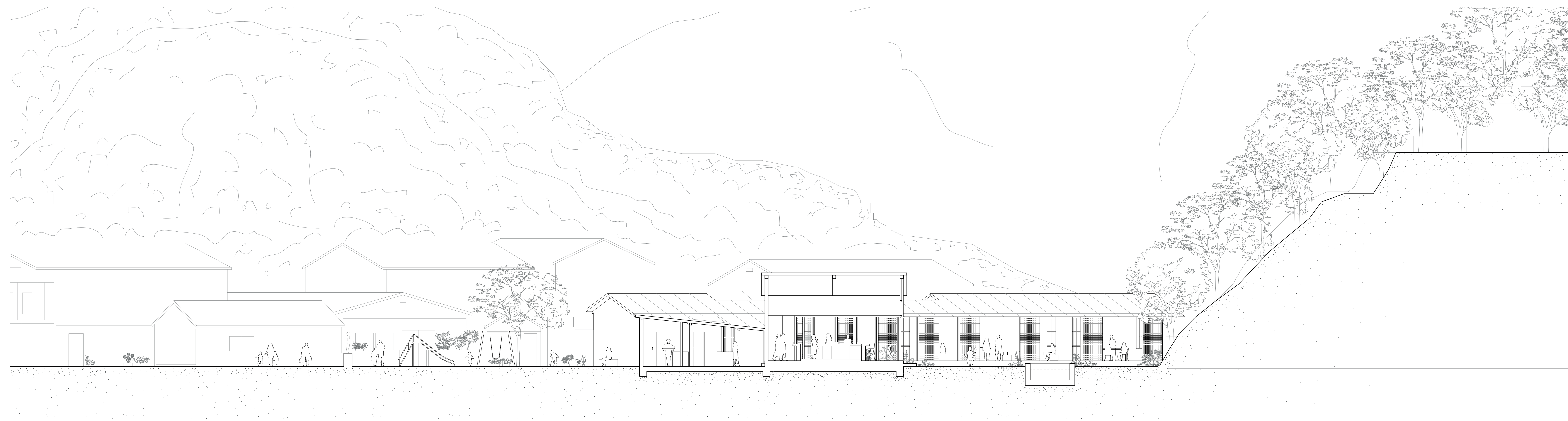
Section BB' 1/100
