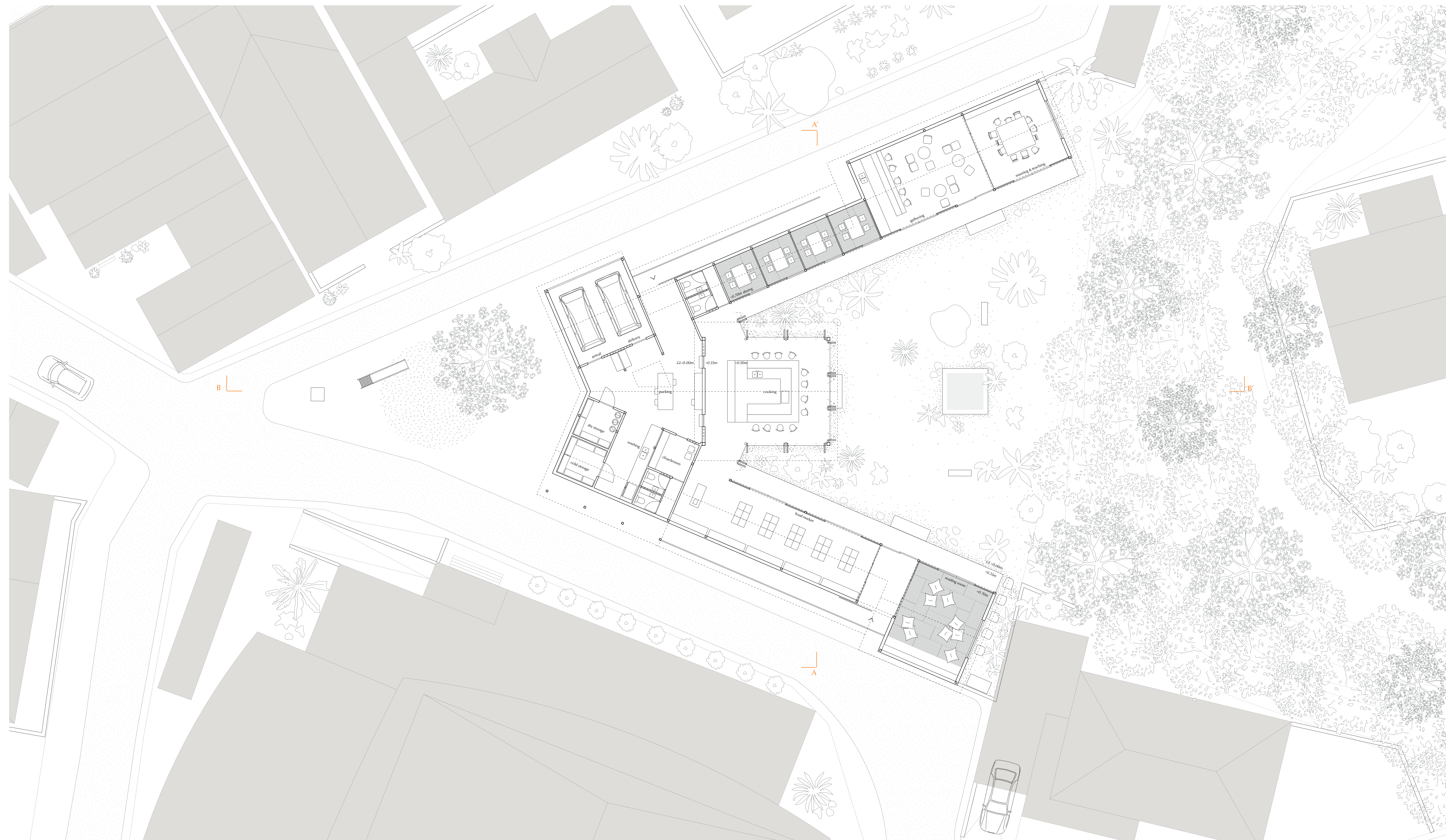
Groundfloor plan 1/100
