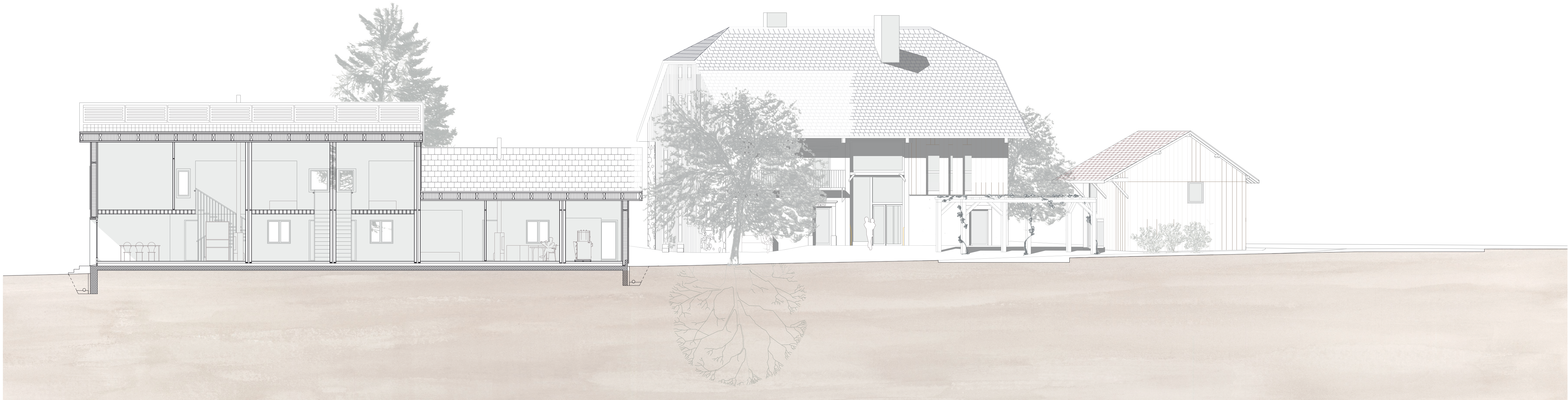
Section aa' 1:100
