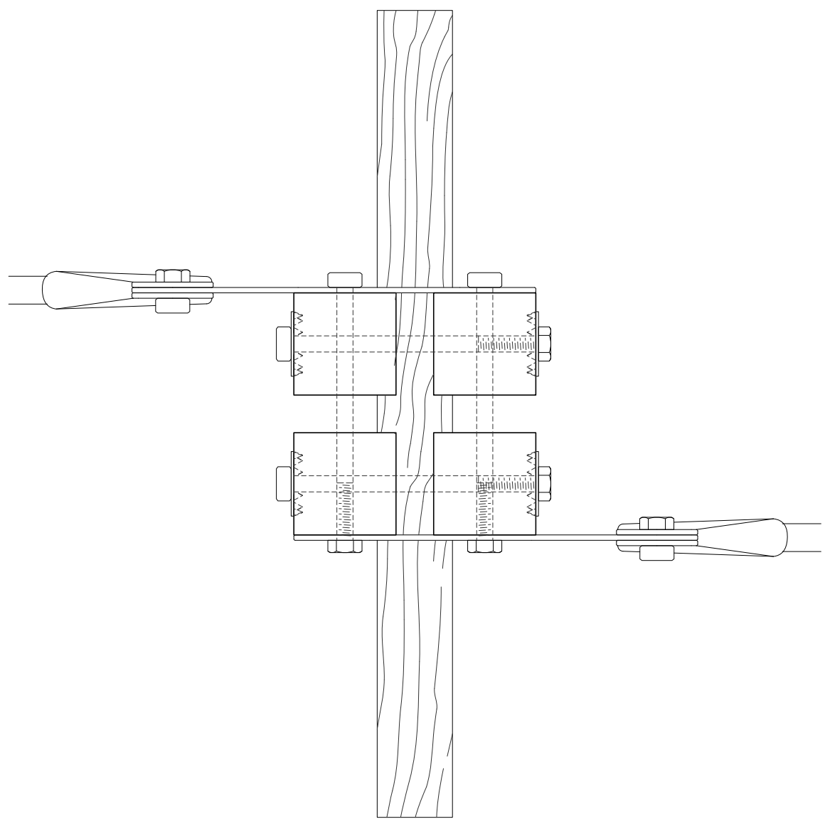
Plan Contreventement
