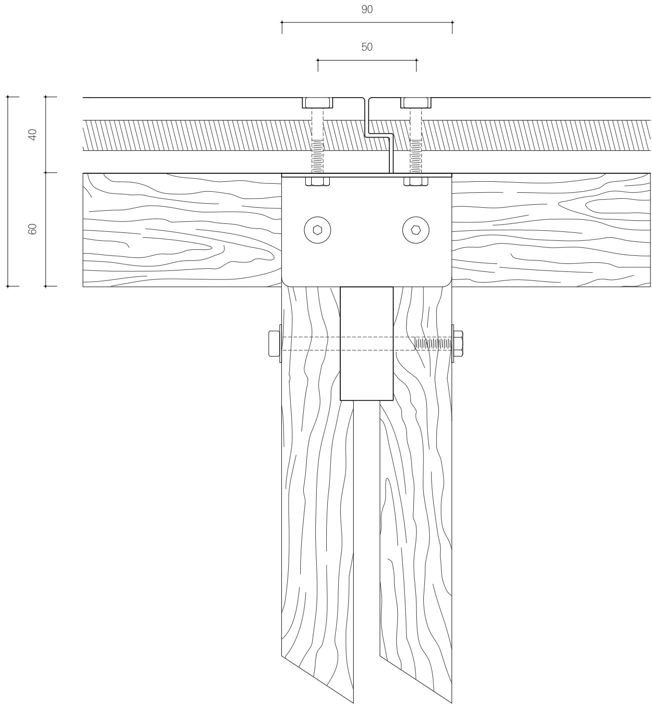
Elevation Plancher
