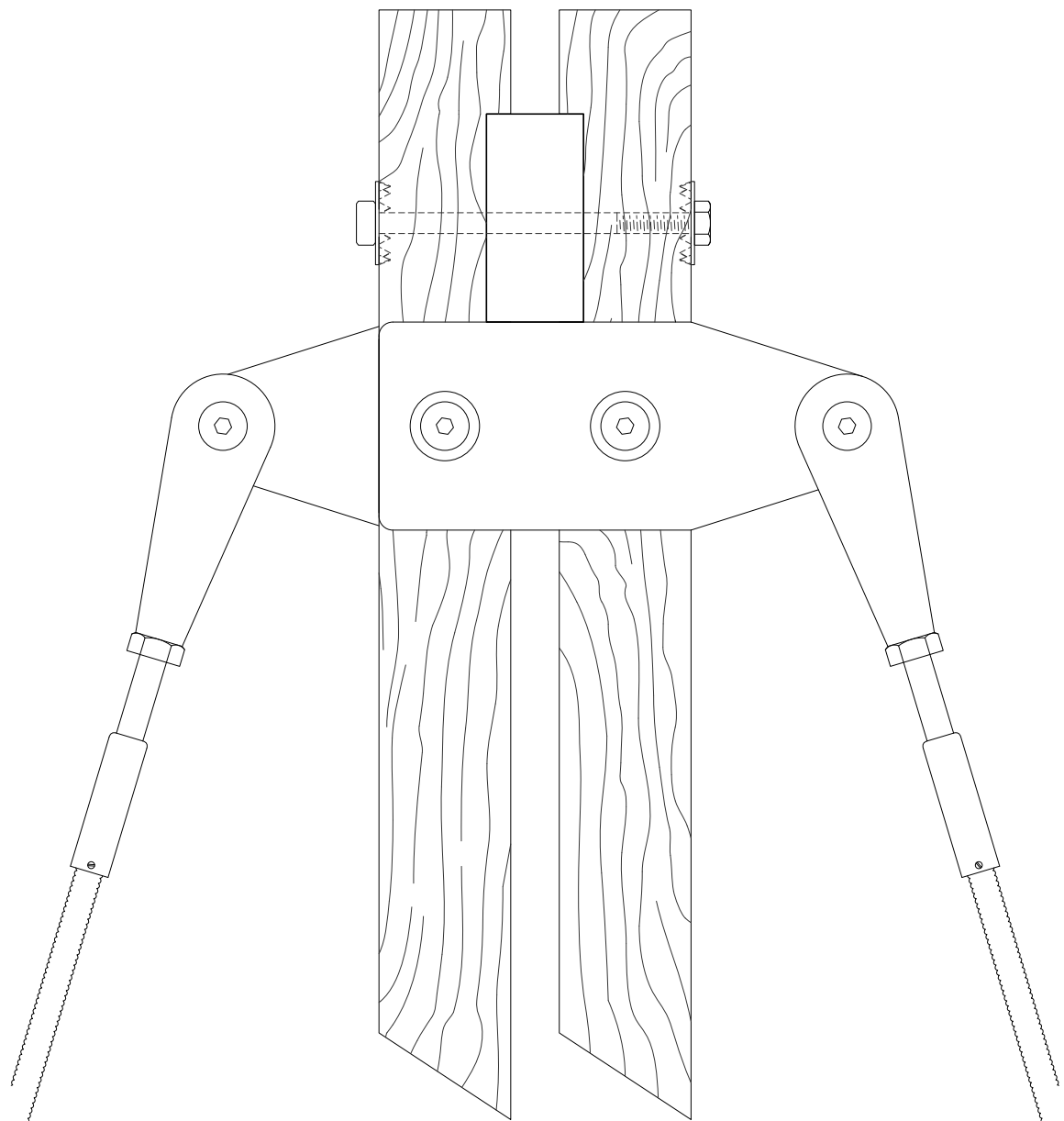
Elevation Contreventement
