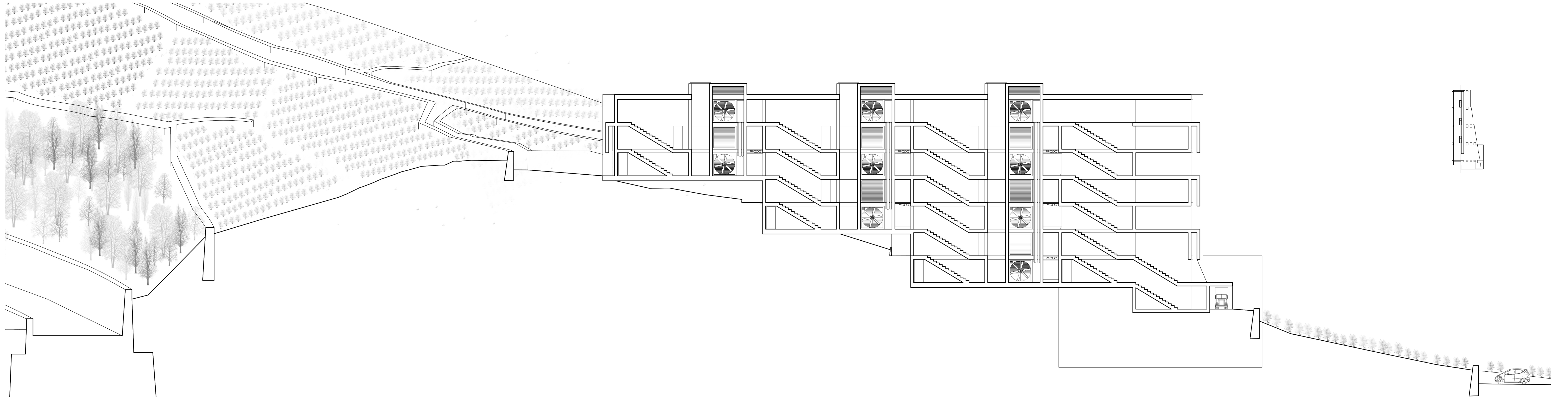
Section long B 1:200
