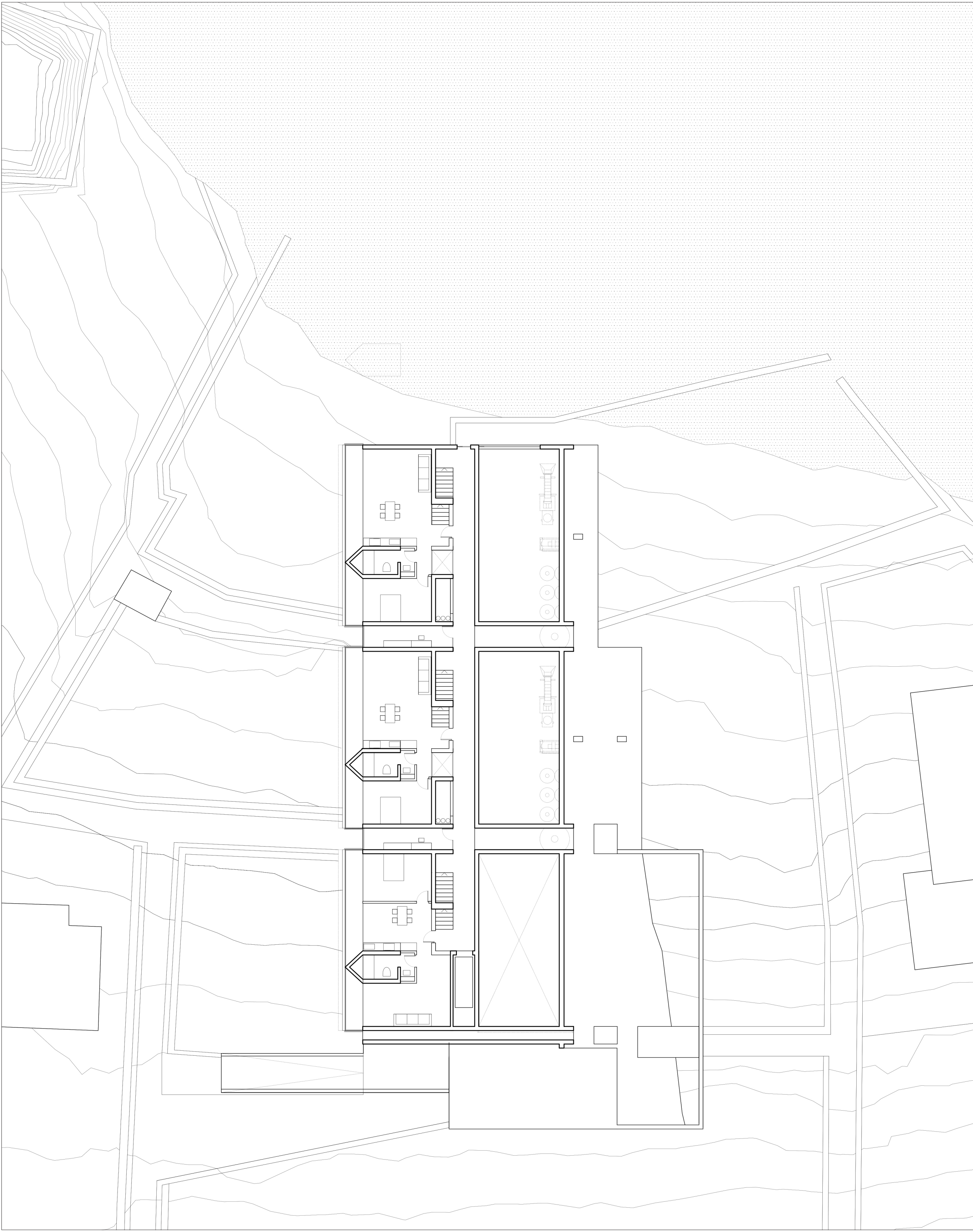
Plan - 2.70m 1:200
