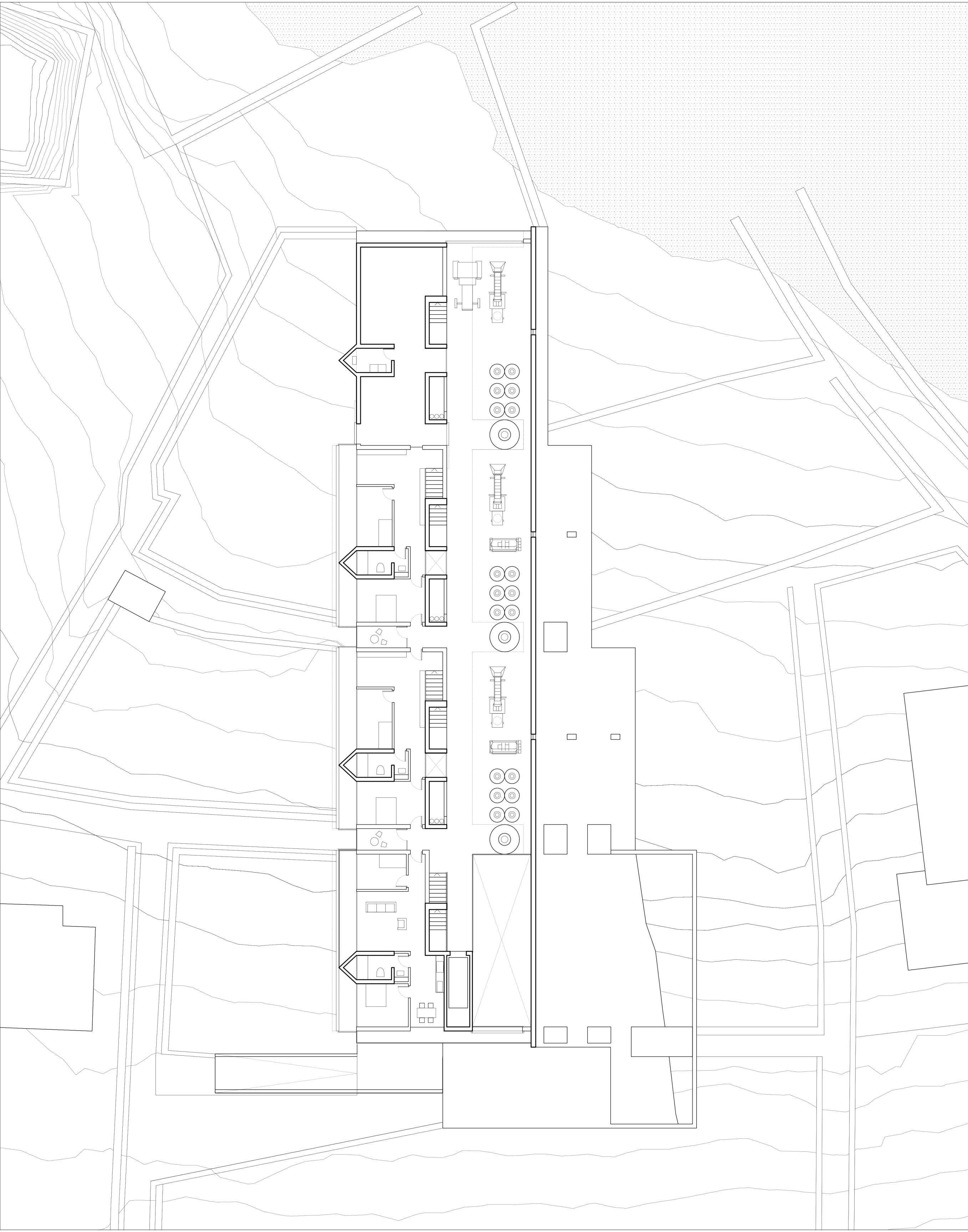
Plan ± 0.00m 1:200
