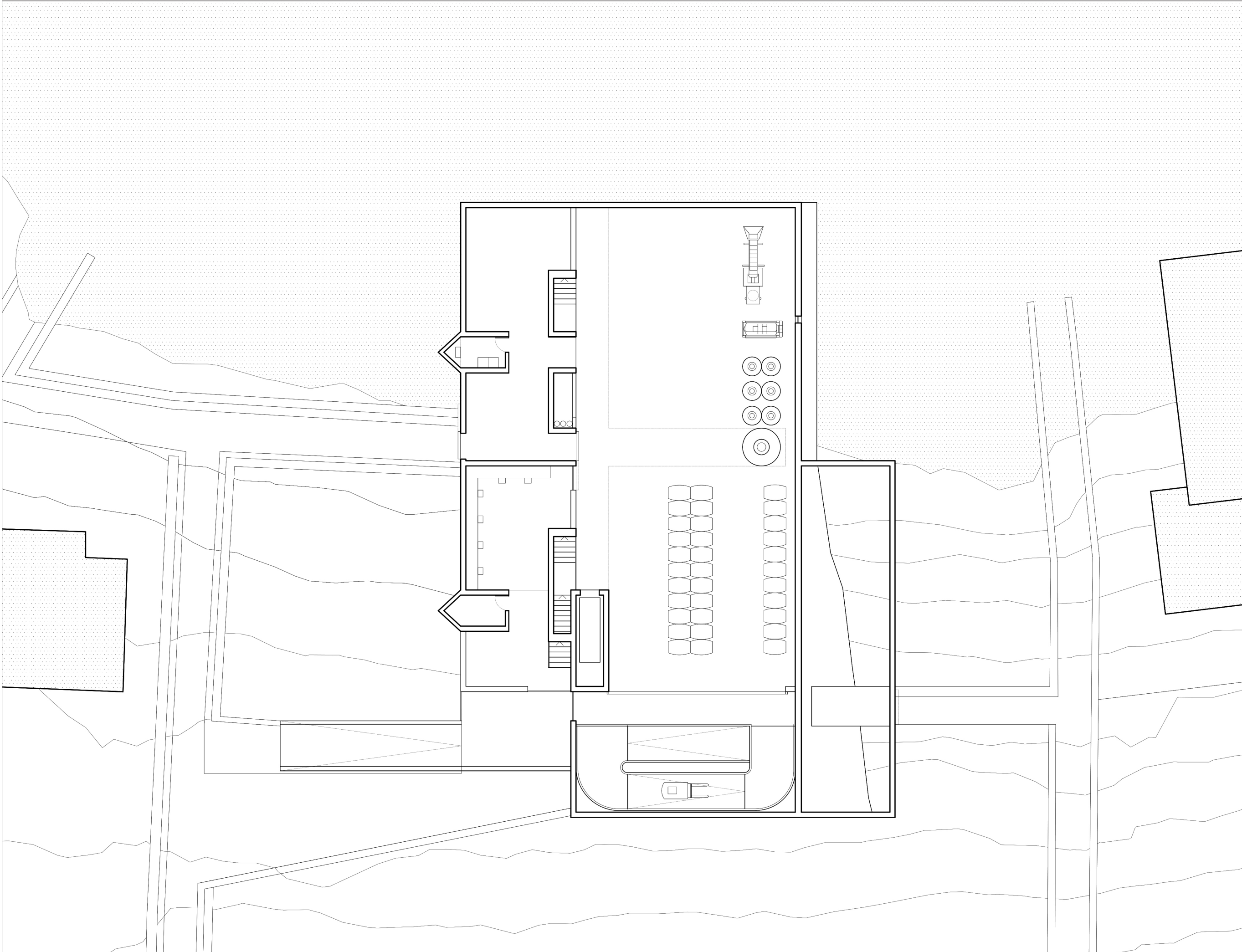
Plan - 10.80m 1:200
