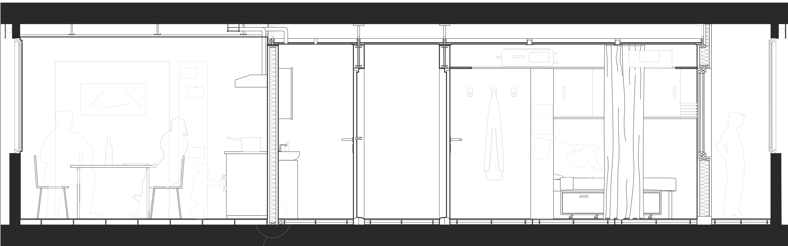
COUPE A FOYER SACONNEX 1_25
