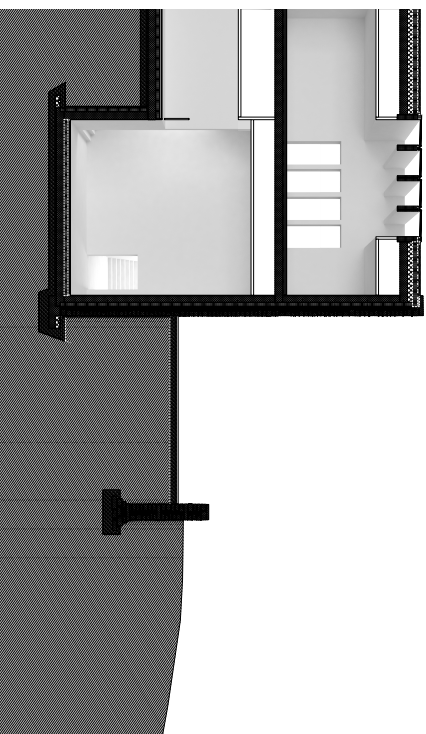
Elevation 55' - 1/50
