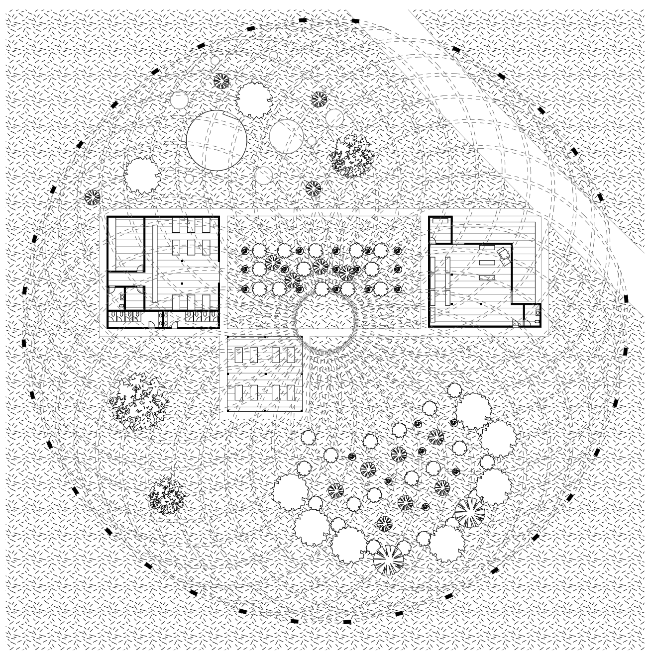
Building plan 1:500
