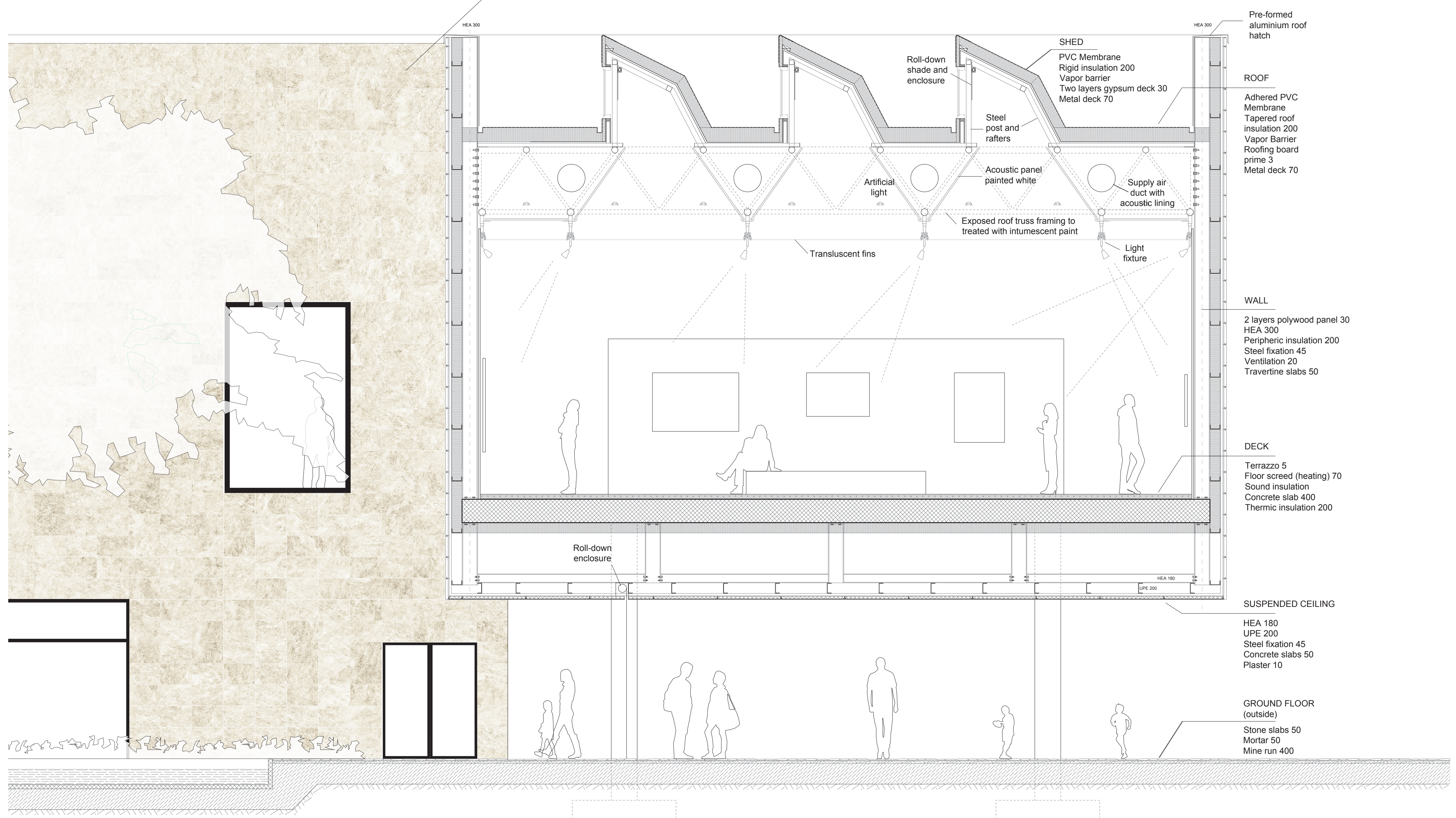
Section through the fine Arts wing 1:50
