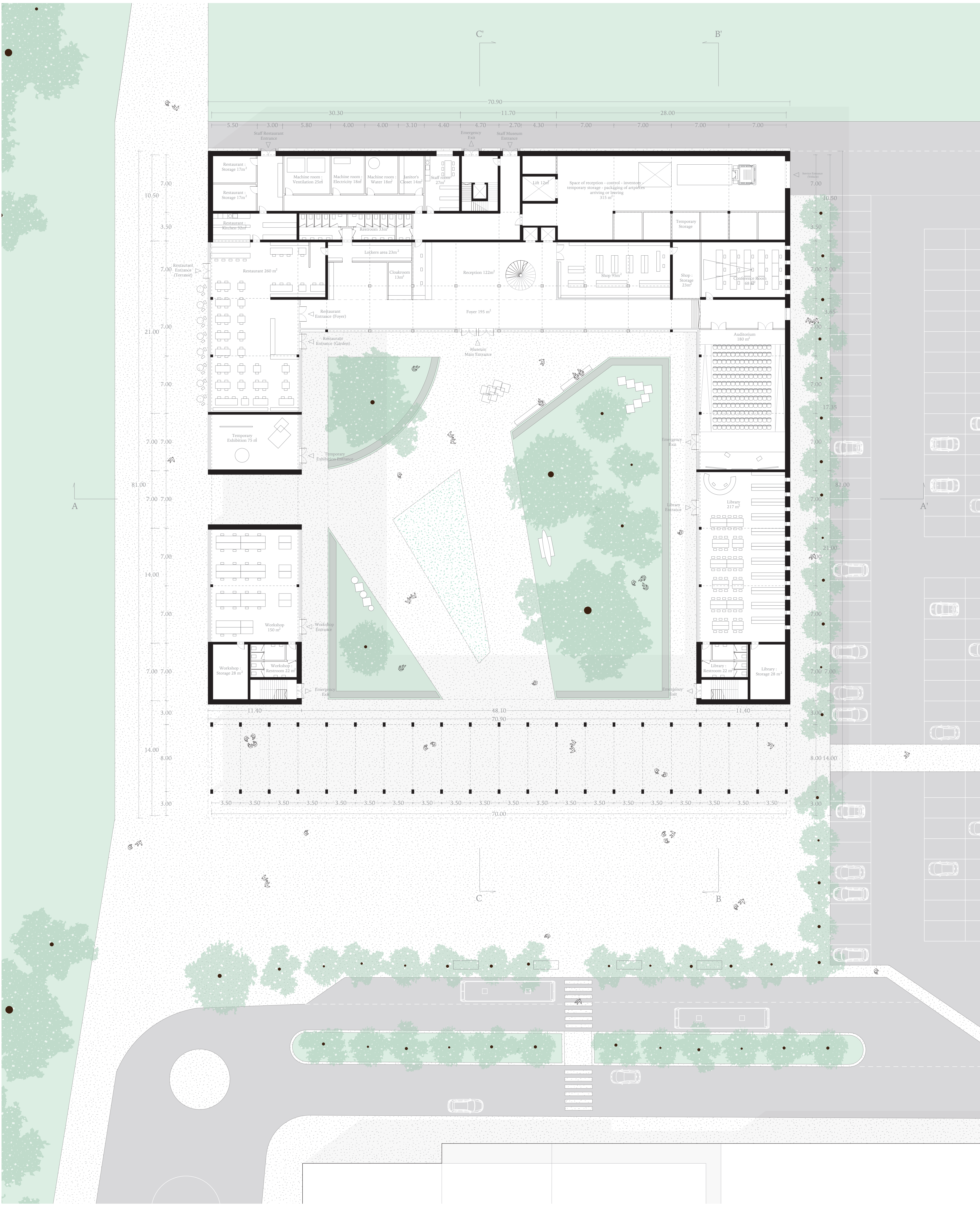
Ground floor plan 1:200
