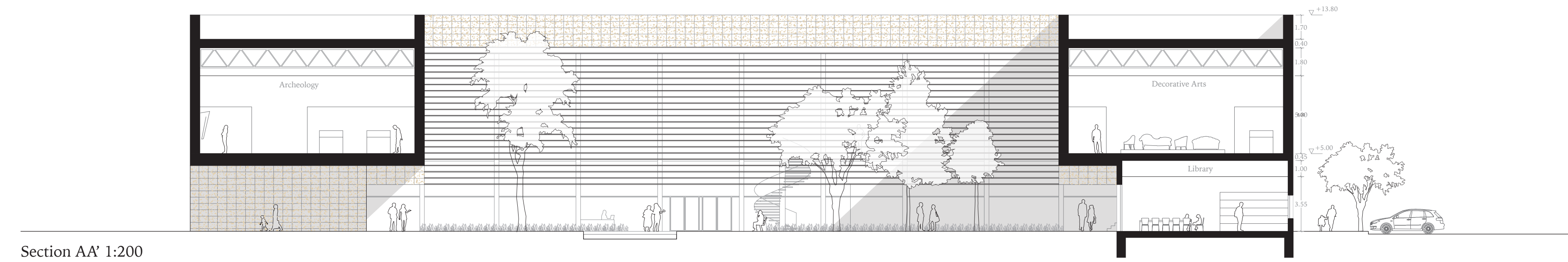
Section AA' 1:200
