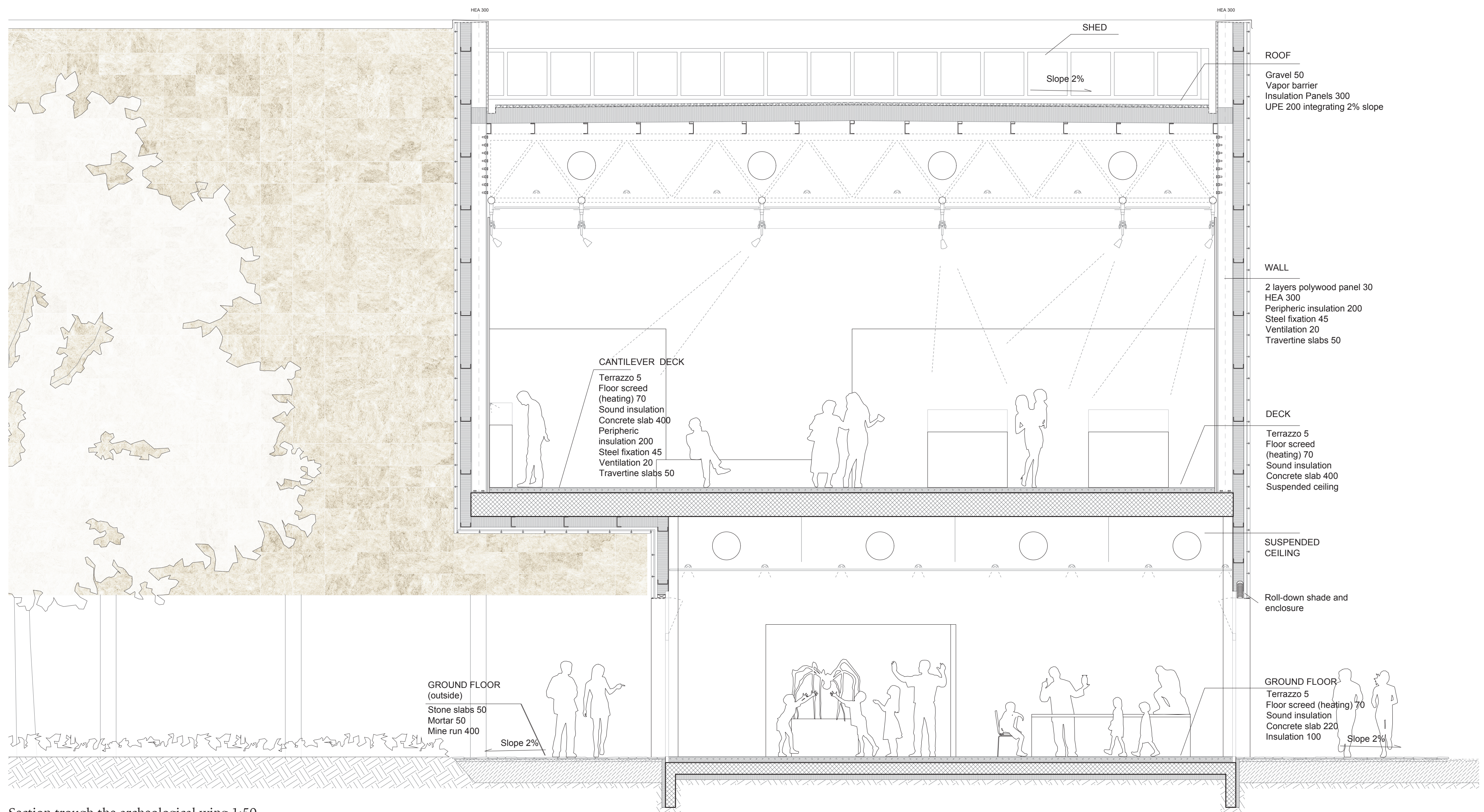
Section through the archeological wing 1:50
