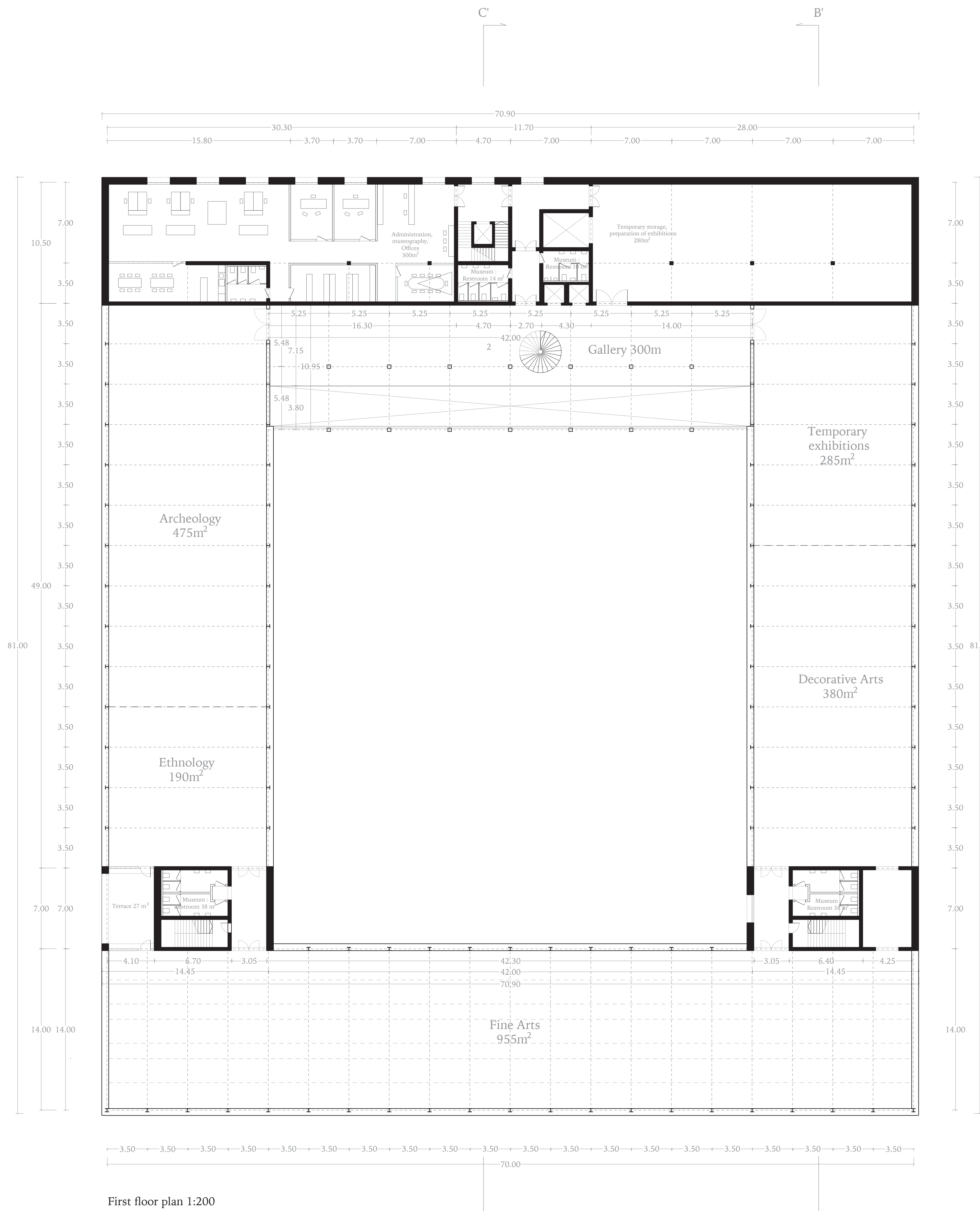
First floor plan 1:200
